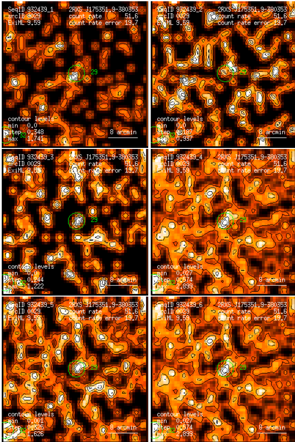
Figure 29: RASS 932439: detection 0029: band rate images, Gaussian filter: (1) PSPC channels 11 – 41, (2) 52 – 90, (3) 91 – 201, (4) 11 – 235, (5) 52 – 201, (6) 11 – 201. Broad band rates in counts/ks. Band rate contour levels in counts/ks/arcmin 2 .
