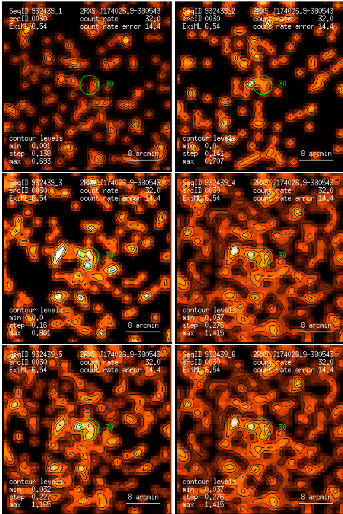
Figure 30: RASS 932439: detection 0030: band rate images, Gaussian filter: (1) PSPC channels 11 – 41, (2) 52 – 90, (3) 91 – 201, (4) 11 – 235, (5) 52 – 201, (6) 11 – 201. Broad band rates in counts/ks. Band rate contour levels in counts/ks/arcmin 2 .
