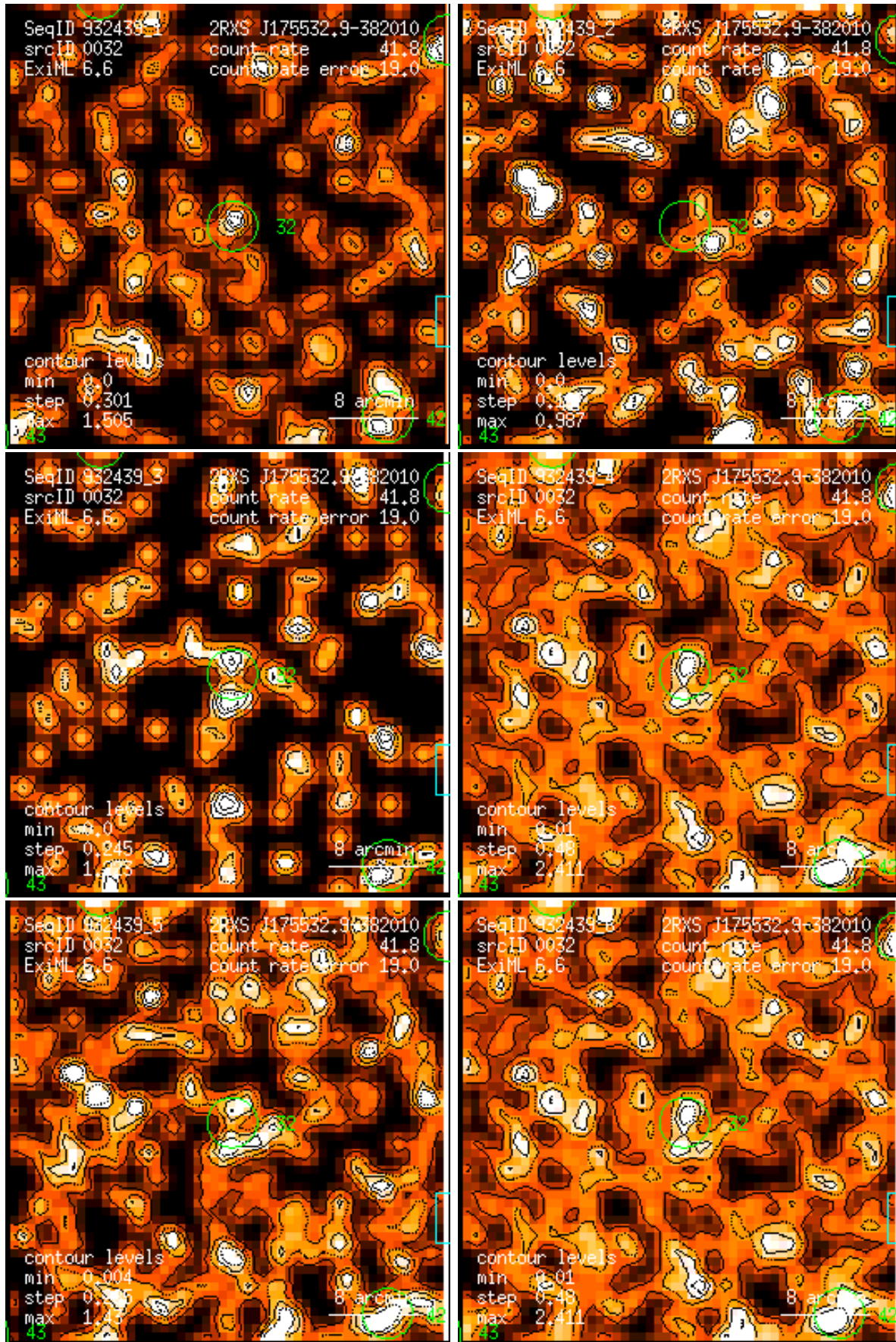
Figure 32: RASS 932439: detection 0032: band rate images, Gaussian filter: (1) PSPC channels 11 – 41, (2) 52 – 90, (3) 91 – 201, (4) 11 – 235, (5) 52 – 201, (6) 11 – 201. Broad band rates in counts/ks. Band rate contour levels in counts/ks/arcmin 2 .
