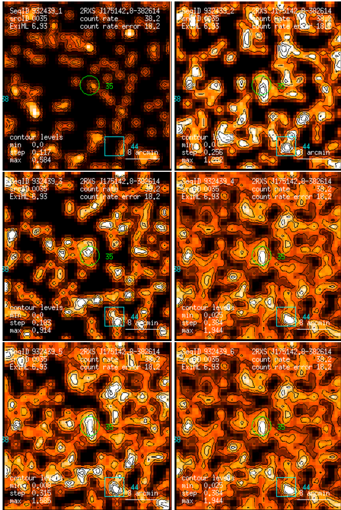
Figure 35: RASS 932439: detection 0035: band rate images, Gaussian filter: (1) PSPC channels 11 – 41, (2) 52 – 90, (3) 91 – 201, (4) 11 – 235, (5) 52 – 201, (6) 11 – 201. Broad band rates in counts/ks. Band rate contour levels in counts/ks/arcmin 2 .
