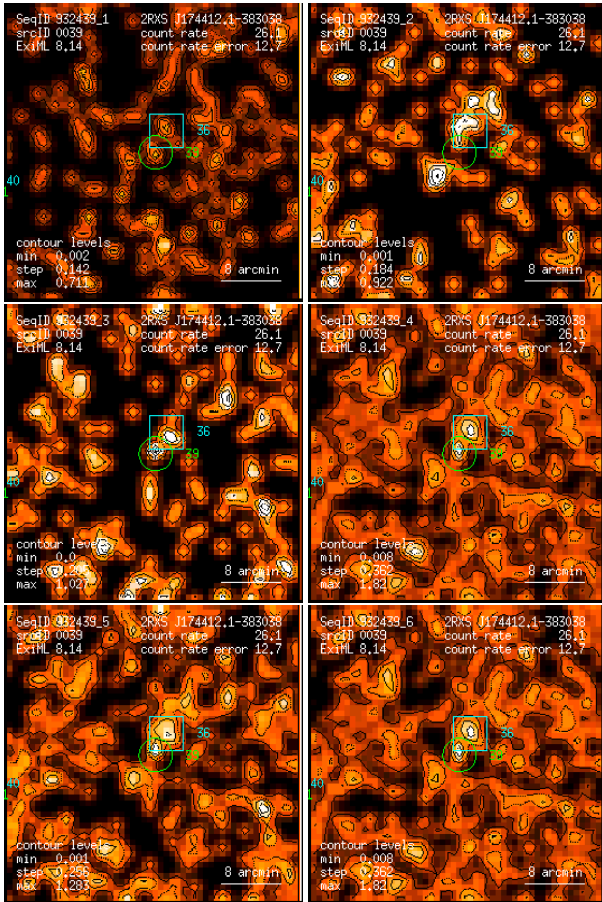
Figure 39: RASS 932439: detection 0039: band rate images, Gaussian filter: (1) PSPC channels 11 – 41, (2) 52 – 90, (3) 91 – 201, (4) 11 – 235, (5) 52 – 201, (6) 11 – 201. Broad band rates in counts/ks. Band rate contour levels in counts/ks/arcmin 2 .
