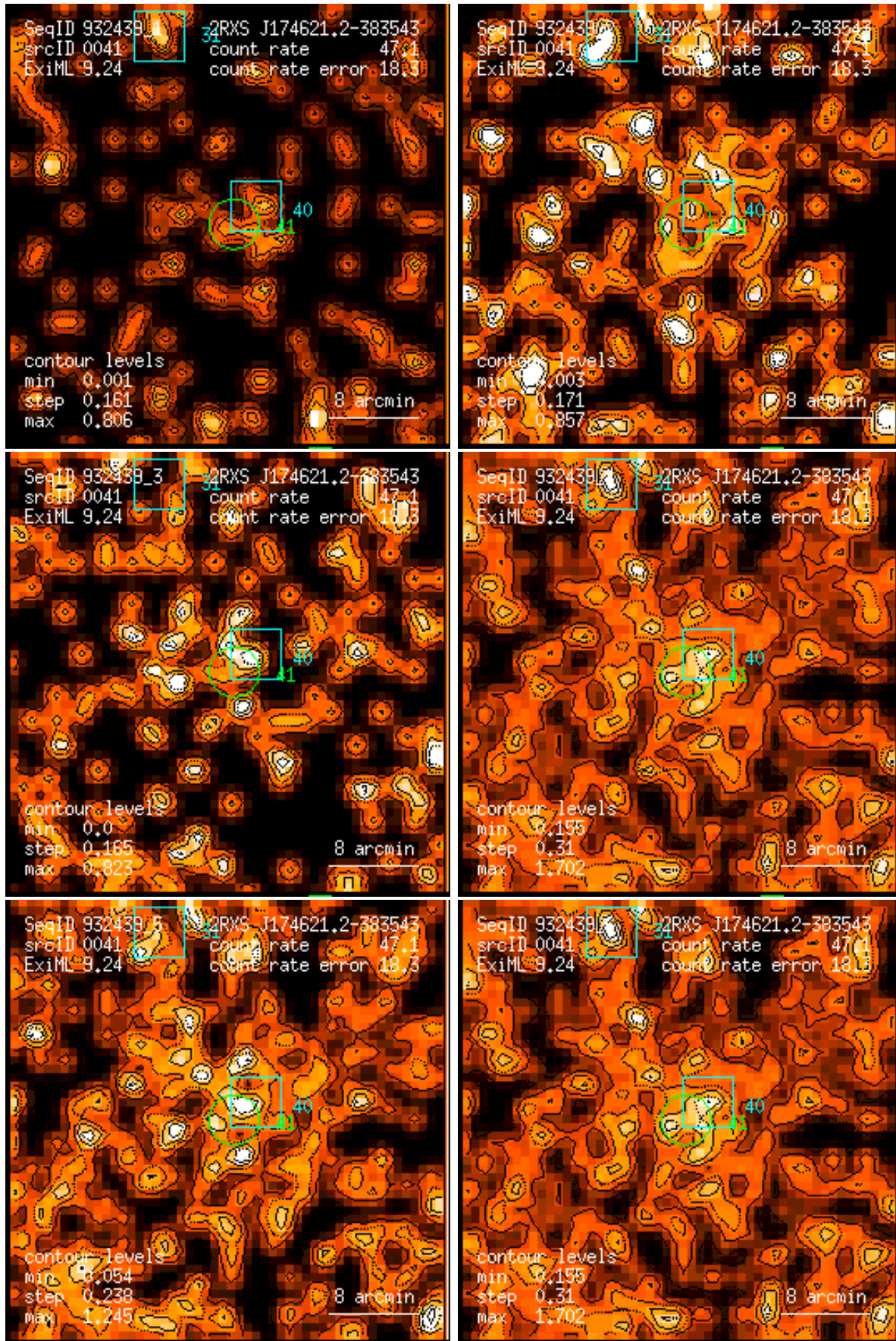
Figure 41: RASS 932439: detection 0041: band rate images, Gaussian filter: (1) PSPC channels 11 – 41, (2) 52 – 90, (3) 91 – 201, (4) 11 – 235, (5) 52 – 201, (6) 11 – 201. Broad band rates in counts/ks. Band rate contour levels in counts/ks/arcmin 2 .
