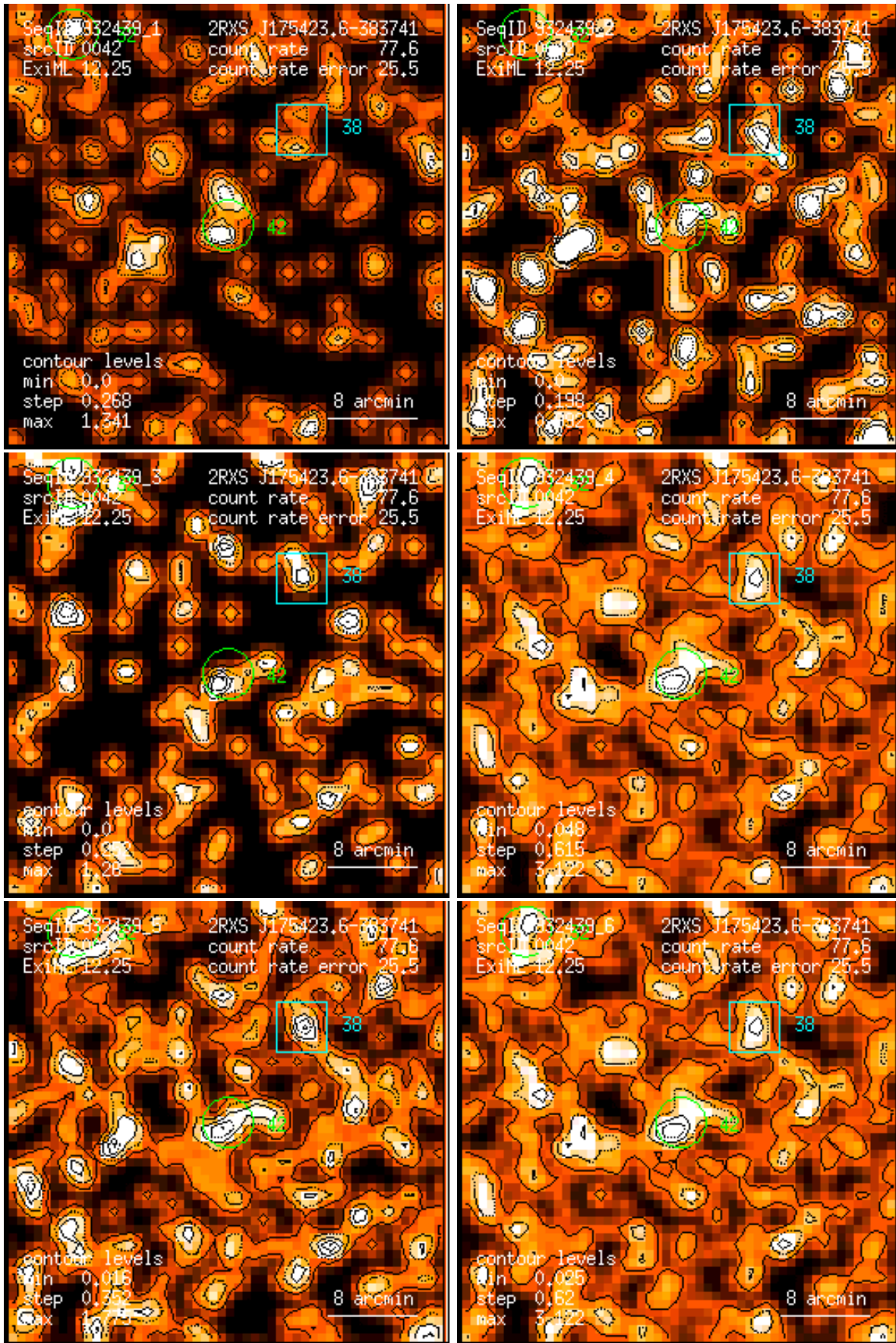
Figure 42: RASS 932439: detection 0042: band rate images, Gaussian filter: (1) PSPC channels 11 – 41, (2) 52 – 90, (3) 91 – 201, (4) 11 – 235, (5) 52 – 201, (6) 11 – 201. Broad band rates in counts/ks. Band rate contour levels in counts/ks/arcmin 2 .
