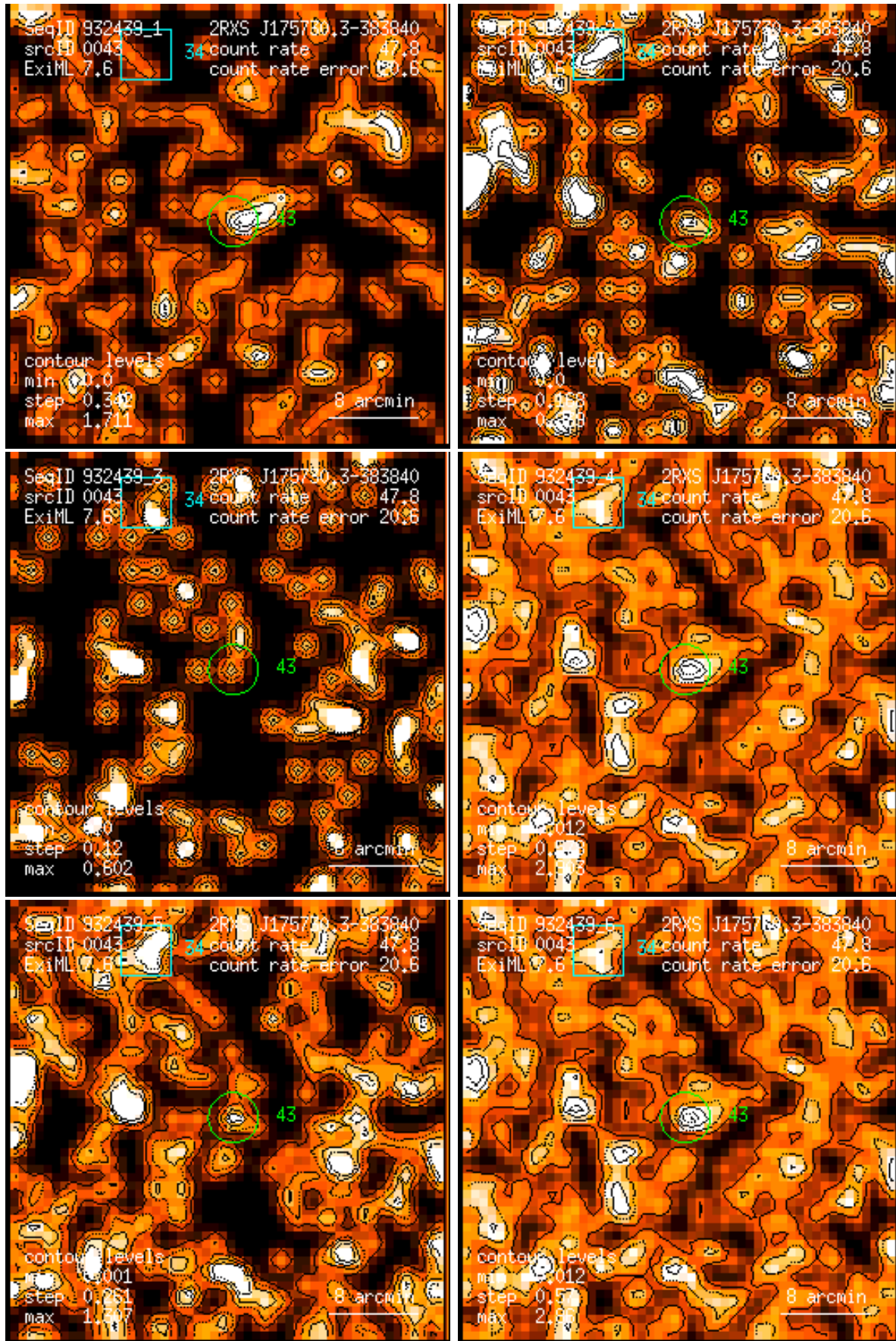
Figure 43: RASS 932439: detection 0043: band rate images, Gaussian filter: (1) PSPC channels 11 – 41, (2) 52 – 90, (3) 91 – 201, (4) 11 – 235, (5) 52 – 201, (6) 11 – 201. Broad band rates in counts/ks. Band rate contour levels in counts/ks/arcmin 2 .
