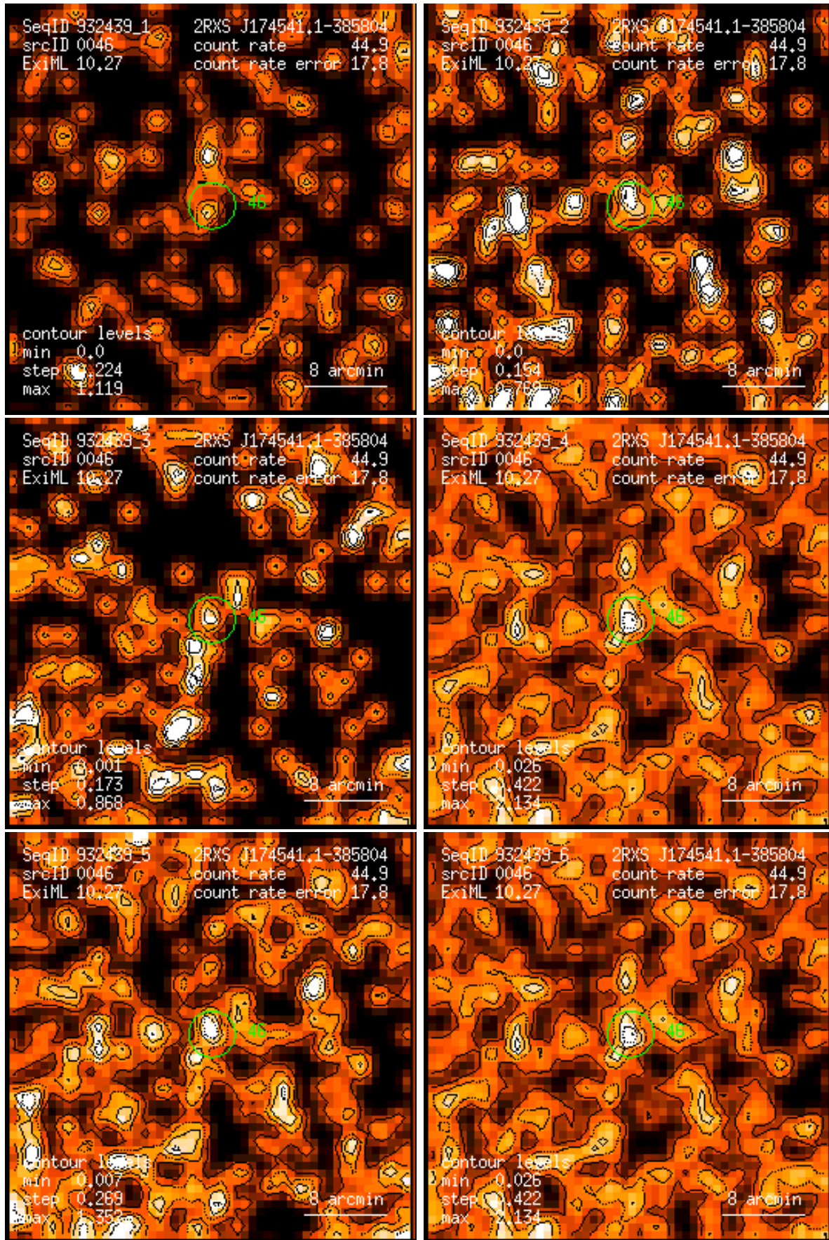
Figure 46: RASS 932439: detection 0046: band rate images, Gaussian filter: (1) PSPC channels 11 – 41, (2) 52 – 90, (3) 91 – 201, (4) 11 – 235, (5) 52 – 201, (6) 11 – 201. Broad band rates in counts/ks. Band rate contour levels in counts/ks/arcmin 2 .
