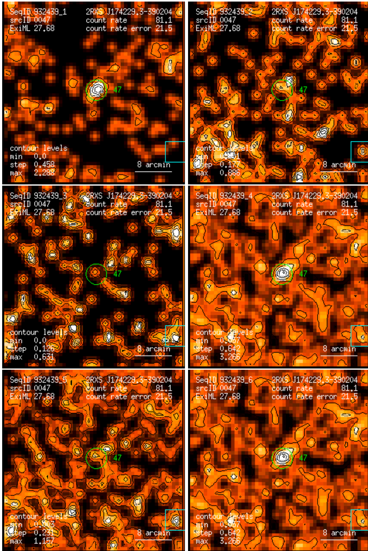
Figure 47: RASS 932439: detection 0047: band rate images, Gaussian filter: (1) PSPC channels 11 – 41, (2) 52 – 90, (3) 91 – 201, (4) 11 – 235, (5) 52 – 201, (6) 11 – 201. Broad band rates in counts/ks. Band rate contour levels in counts/ks/arcmin 2 .
