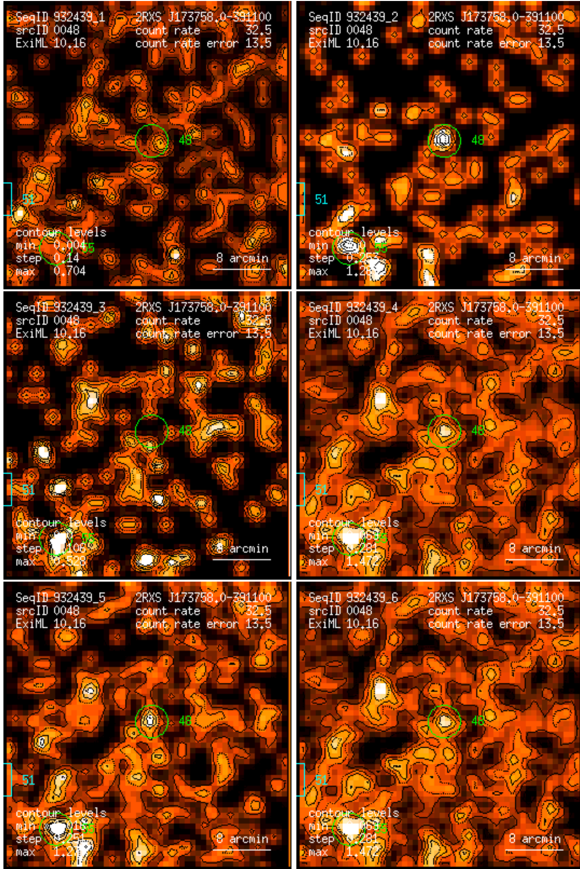
Figure 48: RASS 932439: detection 0048: band rate images, Gaussian filter: (1) PSPC channels 11 – 41, (2) 52 – 90, (3) 91 – 201, (4) 11 – 235, (5) 52 – 201, (6) 11 – 201. Broad band rates in counts/ks. Band rate contour levels in counts/ks/arcmin 2 .
