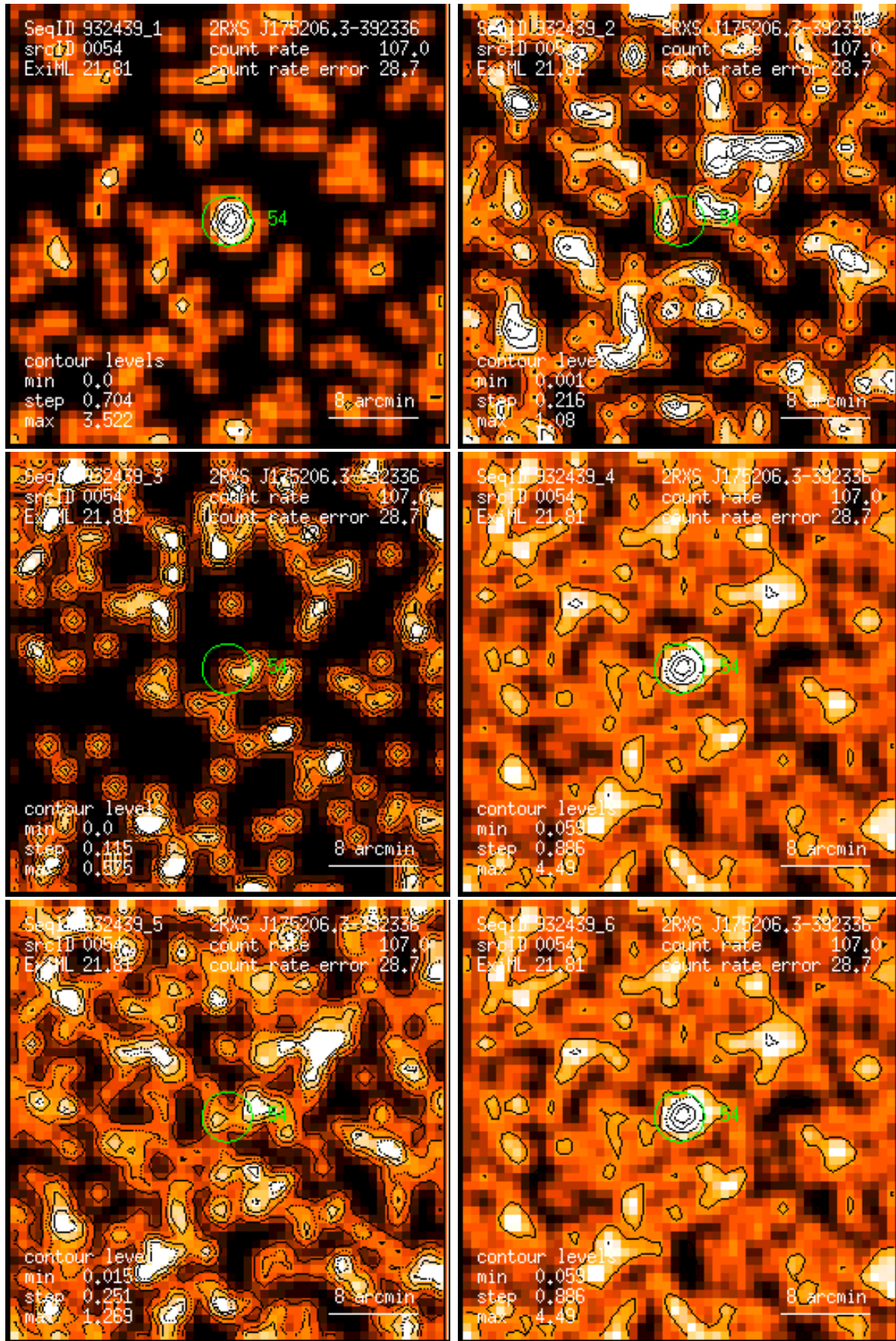
Figure 54: RASS 932439: detection 0054: band rate images, Gaussian filter: (1) PSPC channels 11 – 41, (2) 52 – 90, (3) 91 – 201, (4) 11 – 235, (5) 52 – 201, (6) 11 – 201. Broad band rates in counts/ks. Band rate contour levels in counts/ks/arcmin 2 .
