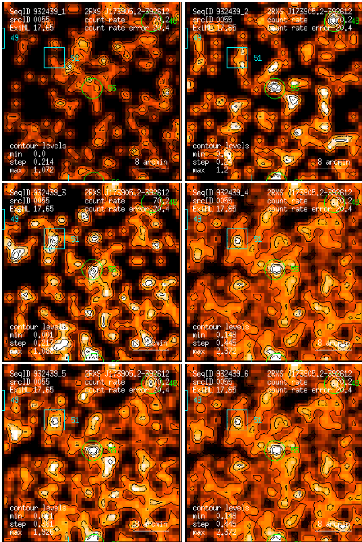
Figure 55: RASS 932439: detection 0055: band rate images, Gaussian filter: (1) PSPC channels 11 – 41, (2) 52 – 90, (3) 91 – 201, (4) 11 – 235, (5) 52 – 201, (6) 11 – 201. Broad band rates in counts/ks. Band rate contour levels in counts/ks/arcmin 2 .
