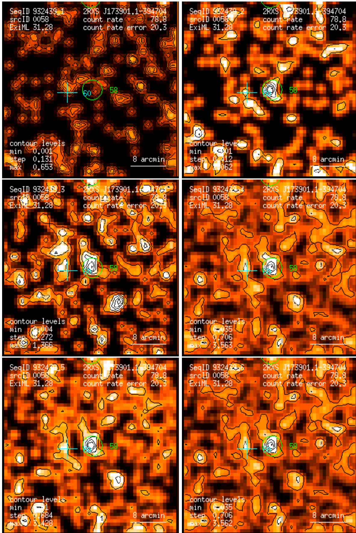
Figure 58: RASS 932439: detection 0058: band rate images, Gaussian filter: (1) PSPC channels 11 – 41, (2) 52 – 90, (3) 91 – 201, (4) 11 – 235, (5) 52 – 201, (6) 11 – 201. Broad band rates in counts/ks. Band rate contour levels in counts/ks/arcmin 2 .
