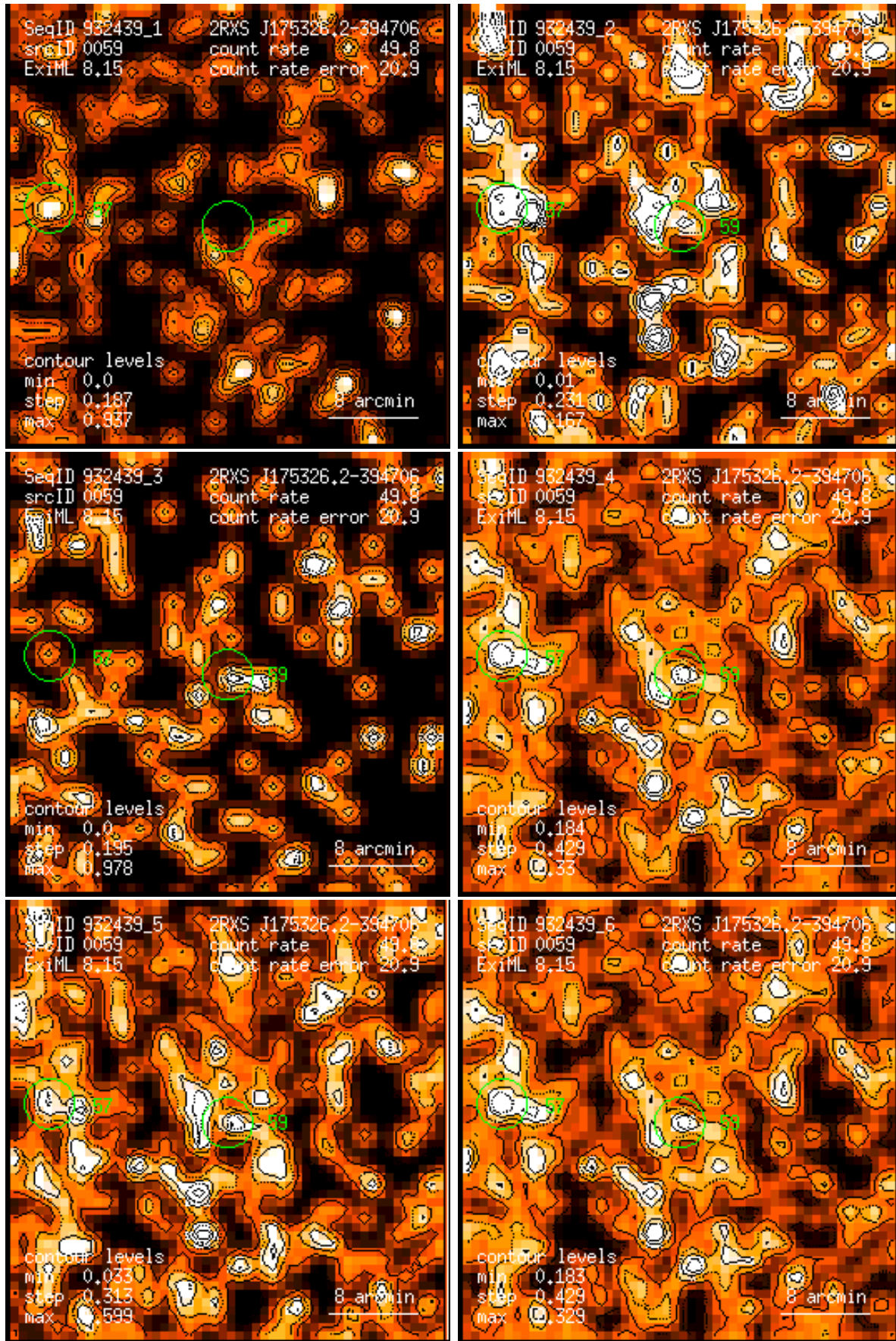
Figure 59: RASS 932439: detection 0059: band rate images, Gaussian filter: (1) PSPC channels 11 – 41, (2) 52 – 90, (3) 91 – 201, (4) 11 – 235, (5) 52 – 201, (6) 11 – 201. Broad band rates in counts/ks. Band rate contour levels in counts/ks/arcmin 2 .
