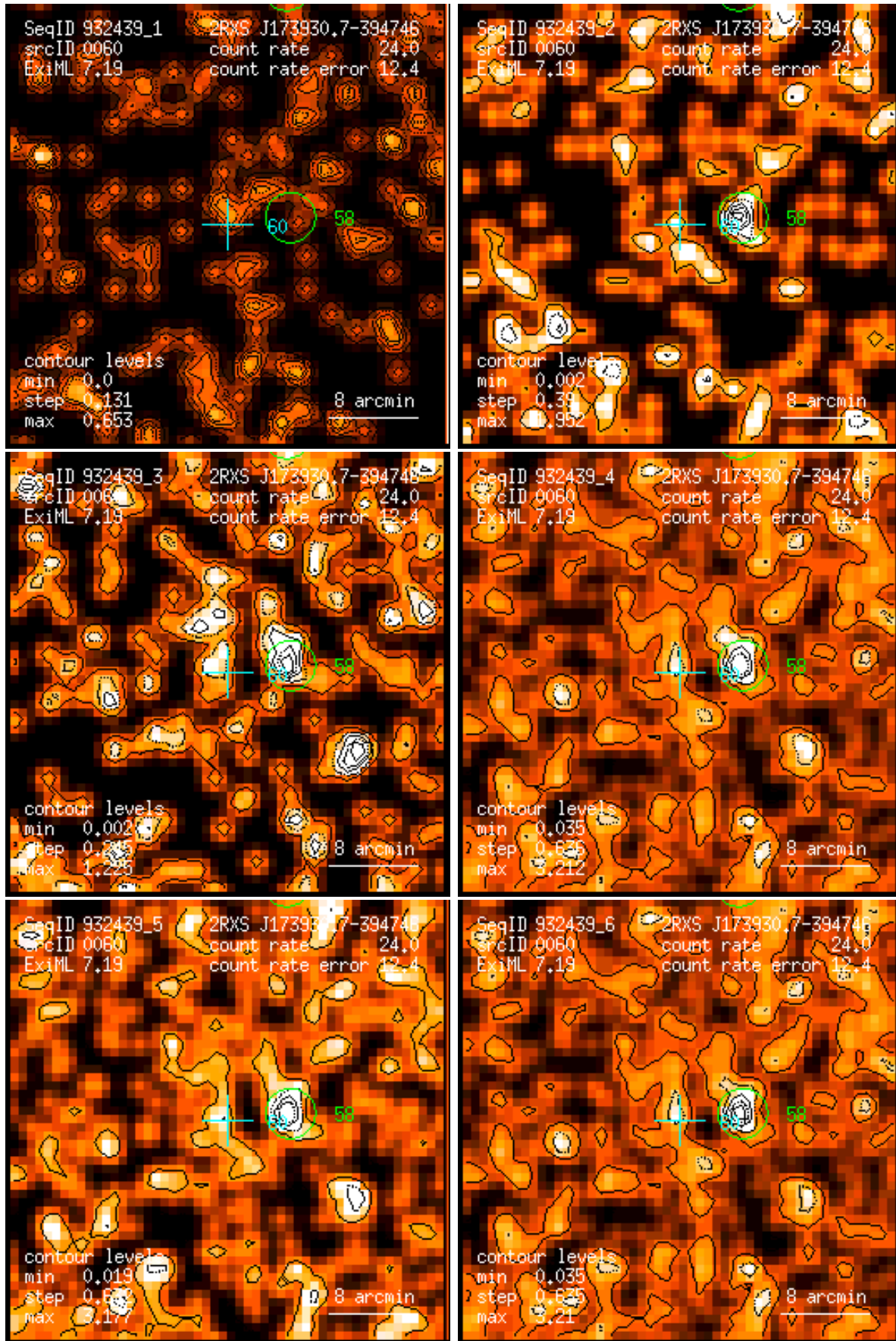
Figure 60: RASS 932439: detection 0060: band rate images, Gaussian filter: (1) PSPC channels 11 – 41, (2) 52 – 90, (3) 91 – 201, (4) 11 – 235, (5) 52 – 201, (6) 11 – 201. Broad band rates in counts/ks. Band rate contour levels in counts/ks/arcmin 2 .
