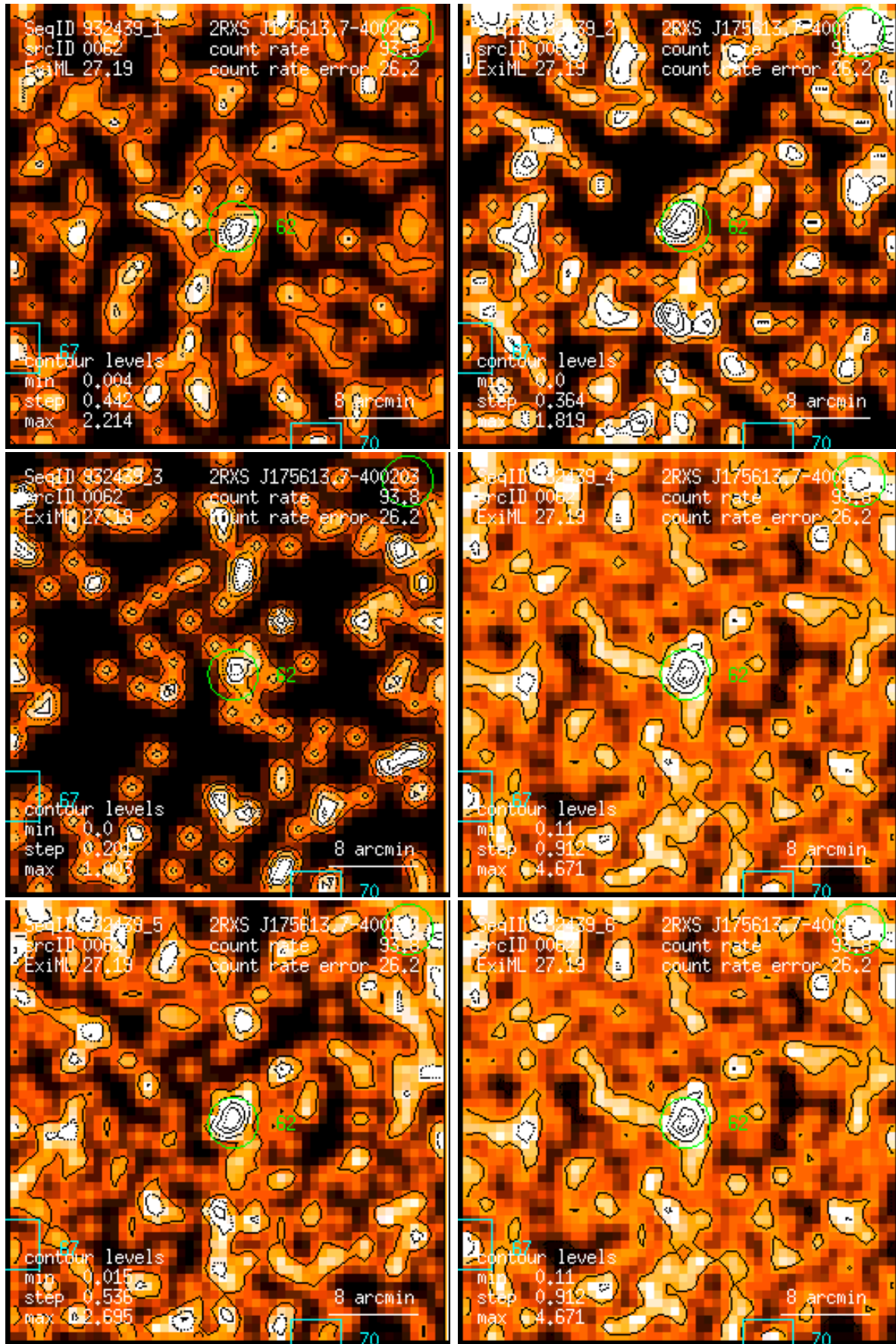
Figure 62: RASS 932439: detection 0062: band rate images, Gaussian filter: (1) PSPC channels 11 – 41, (2) 52 – 90, (3) 91 – 201, (4) 11 – 235, (5) 52 – 201, (6) 11 – 201. Broad band rates in counts/ks. Band rate contour levels in counts/ks/arcmin 2 .
