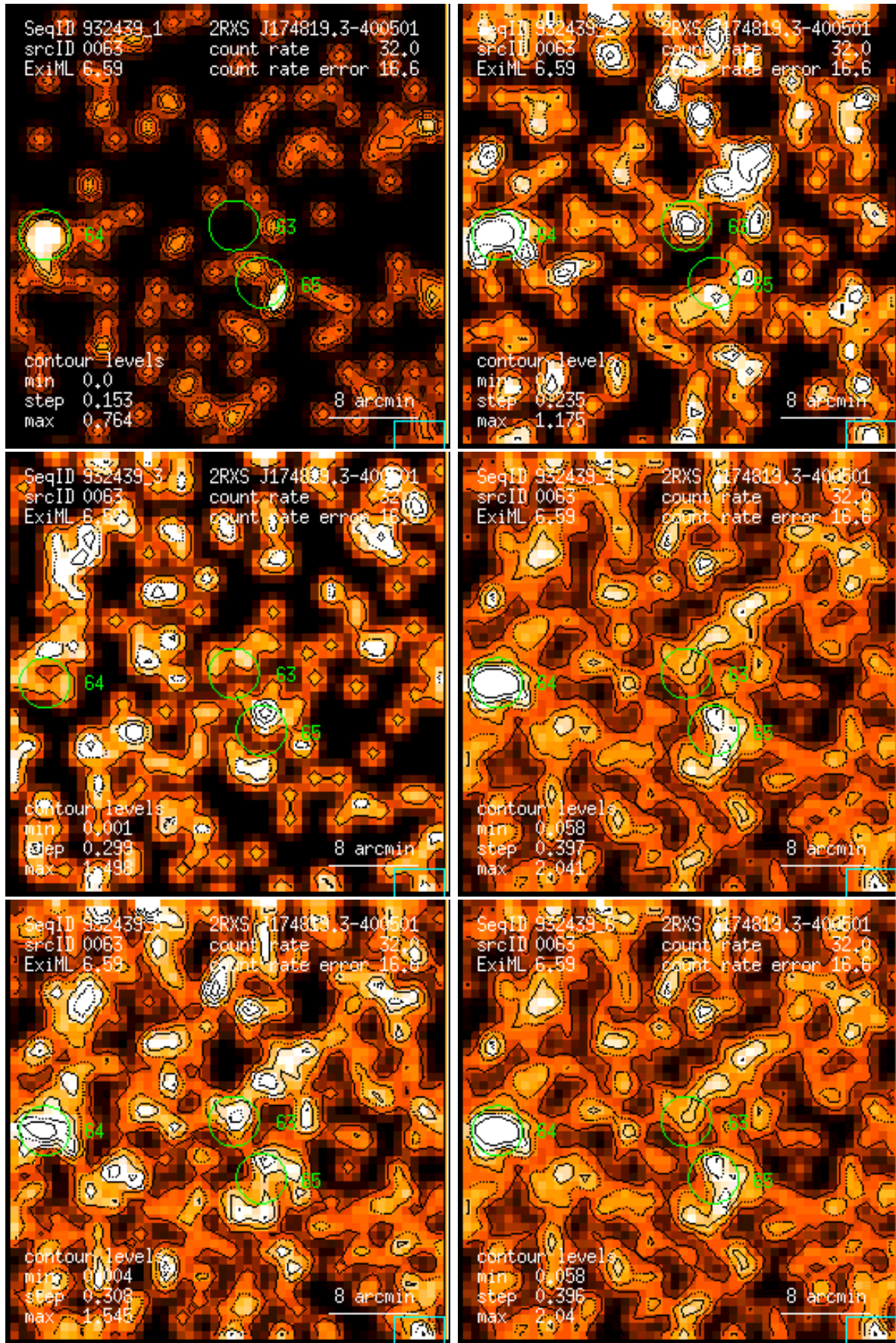
Figure 63: RASS 932439: detection 0063: band rate images, Gaussian filter: (1) PSPC channels 11 – 41, (2) 52 – 90, (3) 91 – 201, (4) 11 – 235, (5) 52 – 201, (6) 11 – 201. Broad band rates in counts/ks. Band rate contour levels in counts/ks/arcmin 2 .
