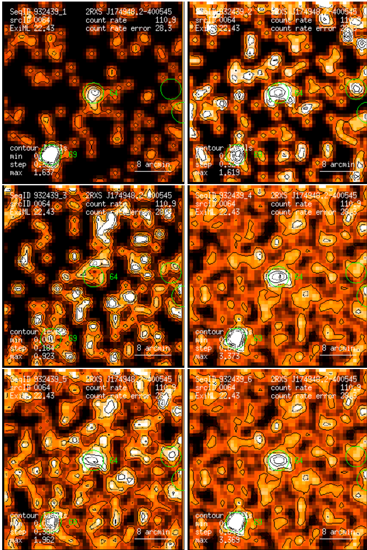
Figure 64: RASS 932439: detection 0064: band rate images, Gaussian filter: (1) PSPC channels 11 – 41, (2) 52 – 90, (3) 91 – 201, (4) 11 – 235, (5) 52 – 201, (6) 11 – 201. Broad band rates in counts/ks. Band rate contour levels in counts/ks/arcmin 2 .
