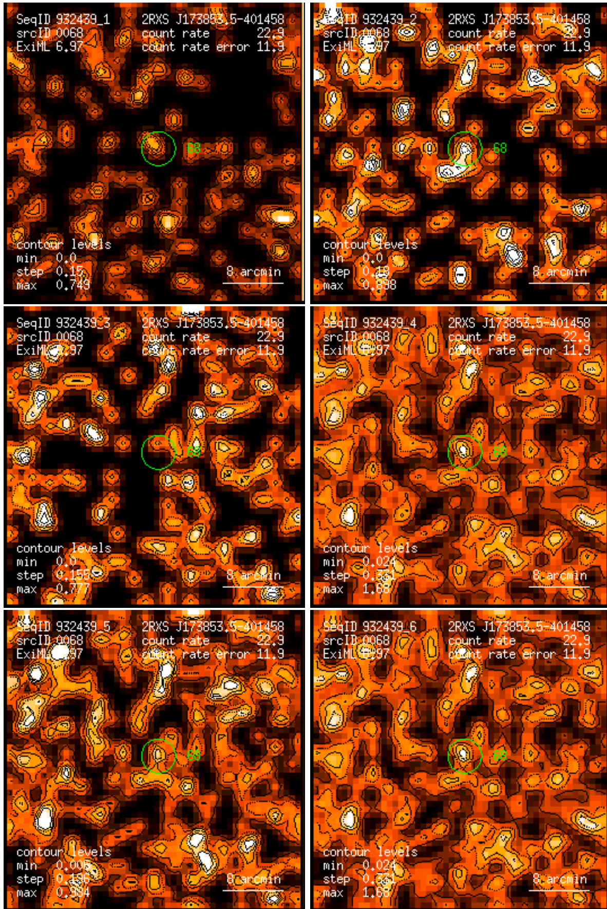
Figure 68: RASS 932439: detection 0068: band rate images, Gaussian filter: (1) PSPC channels 11 – 41, (2) 52 – 90, (3) 91 – 201, (4) 11 – 235, (5) 52 – 201, (6) 11 – 201. Broad band rates in counts/ks. Band rate contour levels in counts/ks/arcmin 2 .
