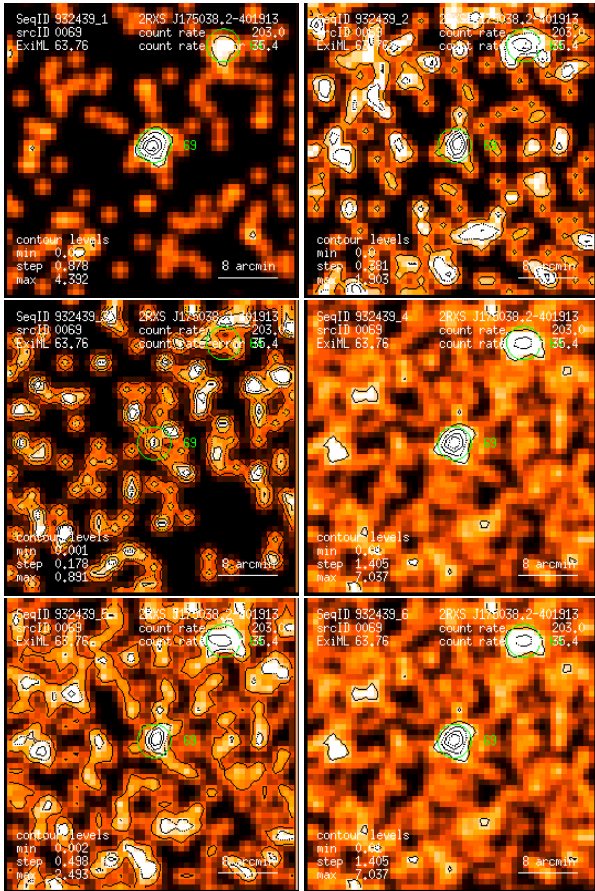
Figure 69: RASS 932439: detection 0069: band rate images, Gaussian filter: (1) PSPC channels 11 – 41, (2) 52 – 90, (3) 91 – 201, (4) 11 – 235, (5) 52 – 201, (6) 11 – 201. Broad band rates in counts/ks. Band rate contour levels in counts/ks/arcmin 2 .
