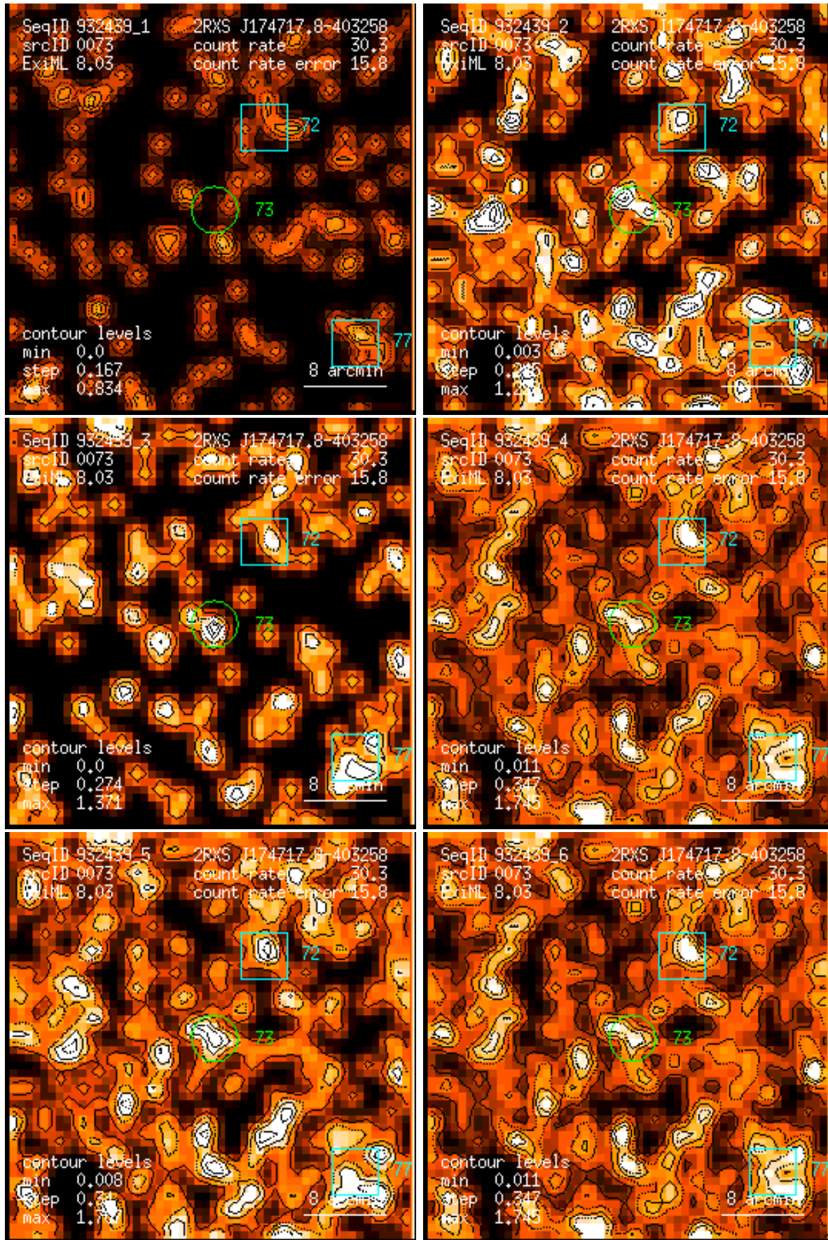
Figure 73: RASS 932439: detection 0073: band rate images, Gaussian filter: (1) PSPC channels 11 – 41, (2) 52 – 90, (3) 91 – 201, (4) 11 – 235, (5) 52 – 201, (6) 11 – 201. Broad band rates in counts/ks. Band rate contour levels in counts/ks/arcmin 2 .
