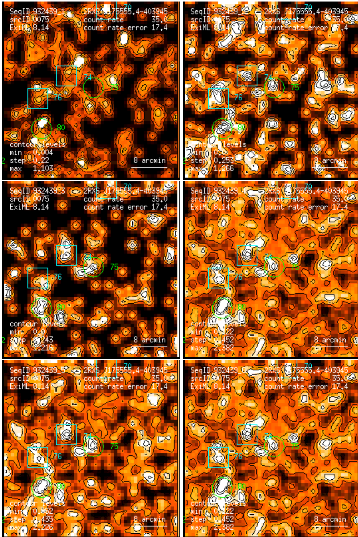
Figure 75: RASS 932439: detection 0075: band rate images, Gaussian filter: (1) PSPC channels 11 – 41, (2) 52 – 90, (3) 91 – 201, (4) 11 – 235, (5) 52 – 201, (6) 11 – 201. Broad band rates in counts/ks. Band rate contour levels in counts/ks/arcmin 2 .
