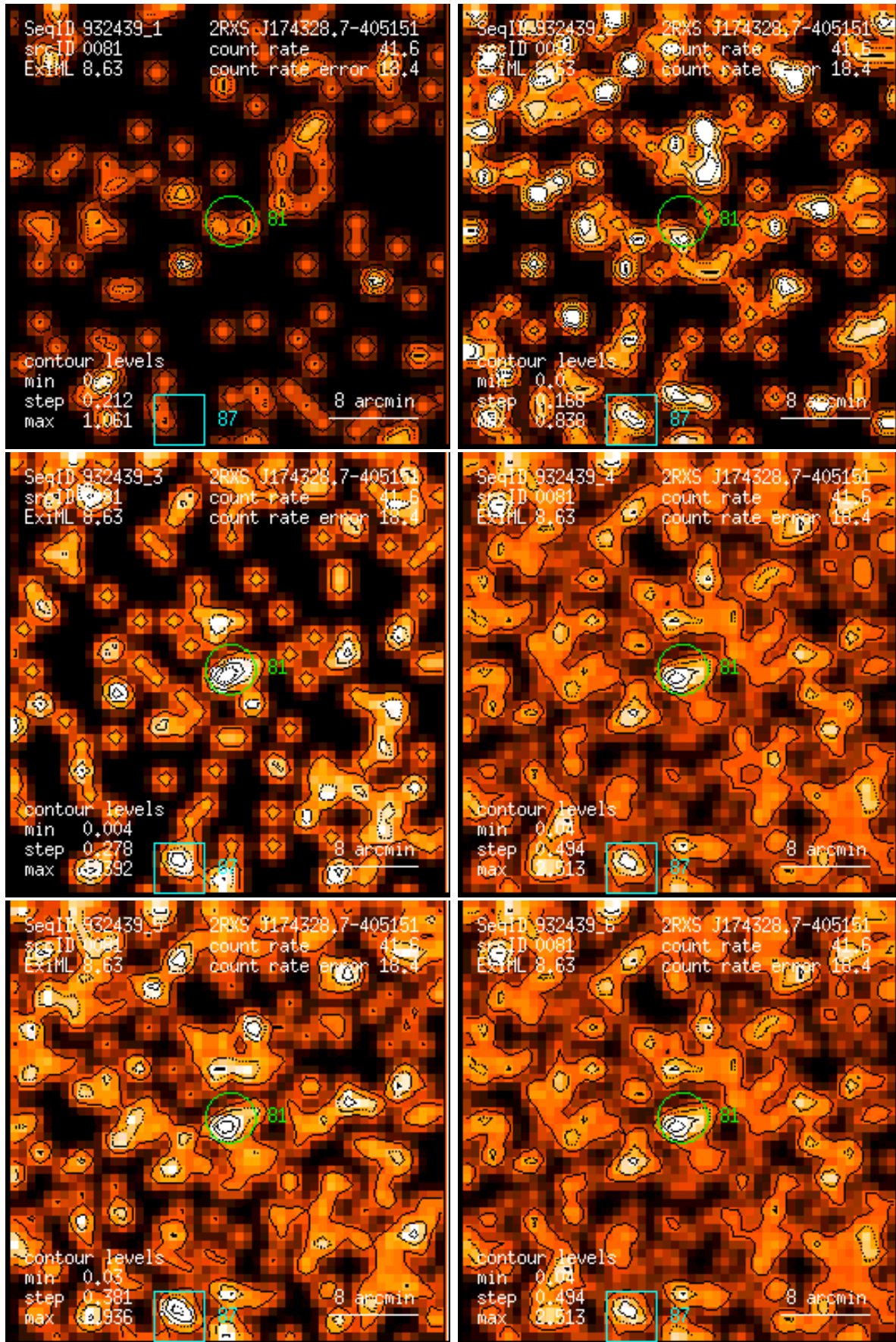
Figure 81: RASS 932439: detection 0081: band rate images, Gaussian filter: (1) PSPC channels 11 – 41, (2) 52 – 90, (3) 91 – 201, (4) 11 – 235, (5) 52 – 201, (6) 11 – 201. Broad band rates in counts/ks. Band rate contour levels in counts/ks/arcmin 2 .
