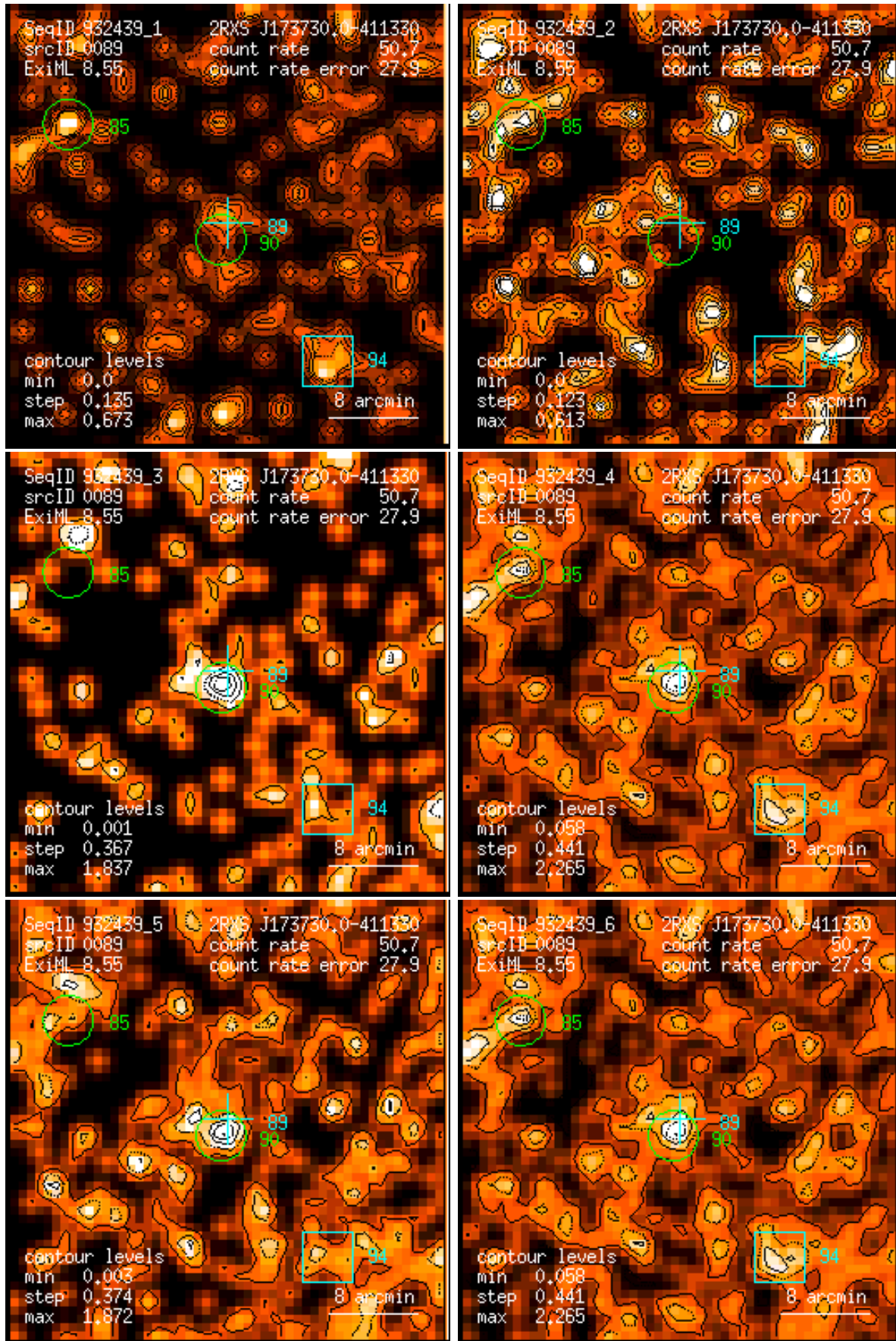
Figure 89: RASS 932439: detection 0089: band rate images, Gaussian filter: (1) PSPC channels 11 – 41, (2) 52 – 90, (3) 91 – 201, (4) 11 – 235, (5) 52 – 201, (6) 11 – 201. Broad band rates in counts/ks. Band rate contour levels in counts/ks/arcmin 2 .
