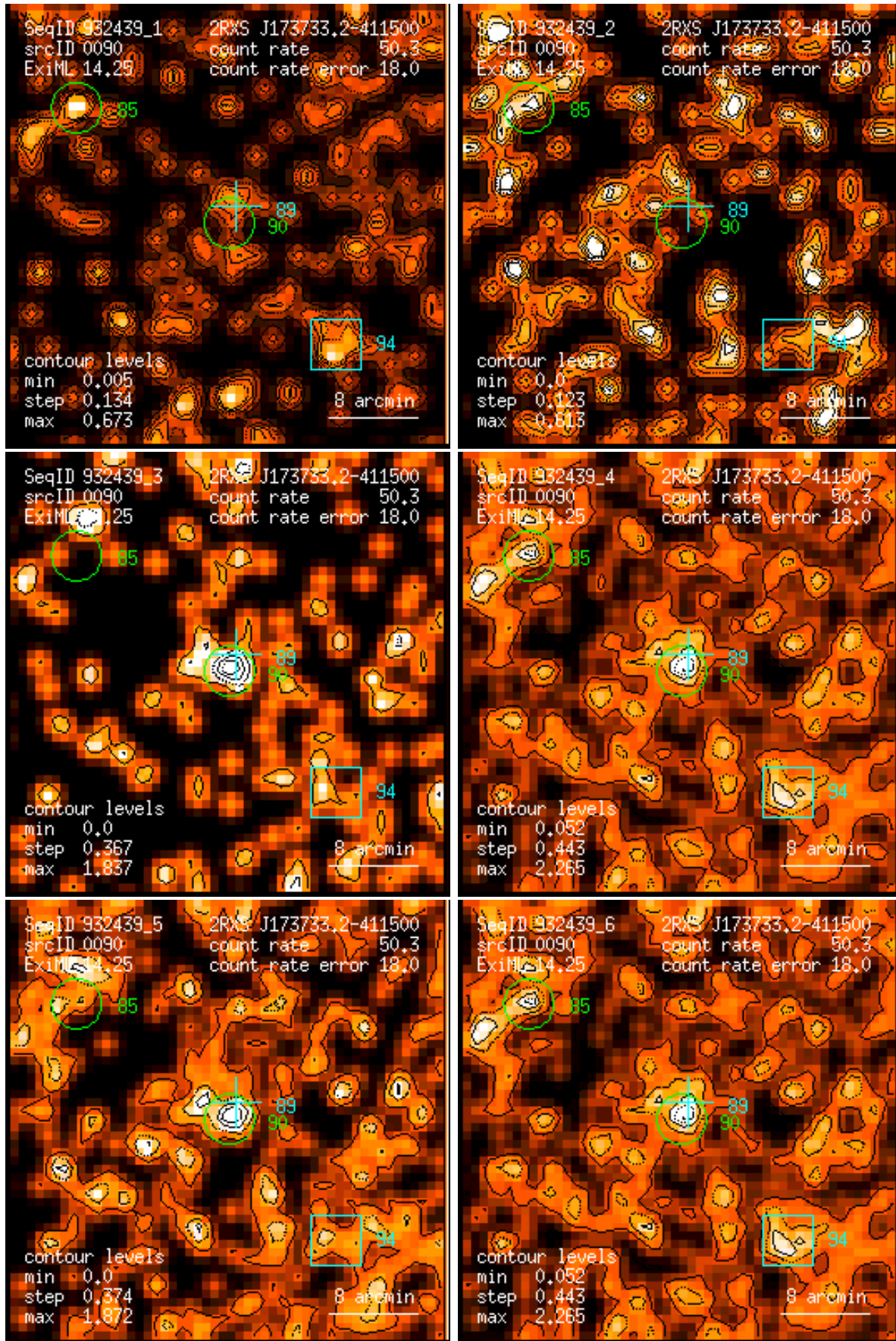
Figure 90: RASS 932439: detection 0090: band rate images, Gaussian filter: (1) PSPC channels 11 – 41, (2) 52 – 90, (3) 91 – 201, (4) 11 – 235, (5) 52 – 201, (6) 11 – 201. Broad band rates in counts/ks. Band rate contour levels in counts/ks/arcmin 2 .
