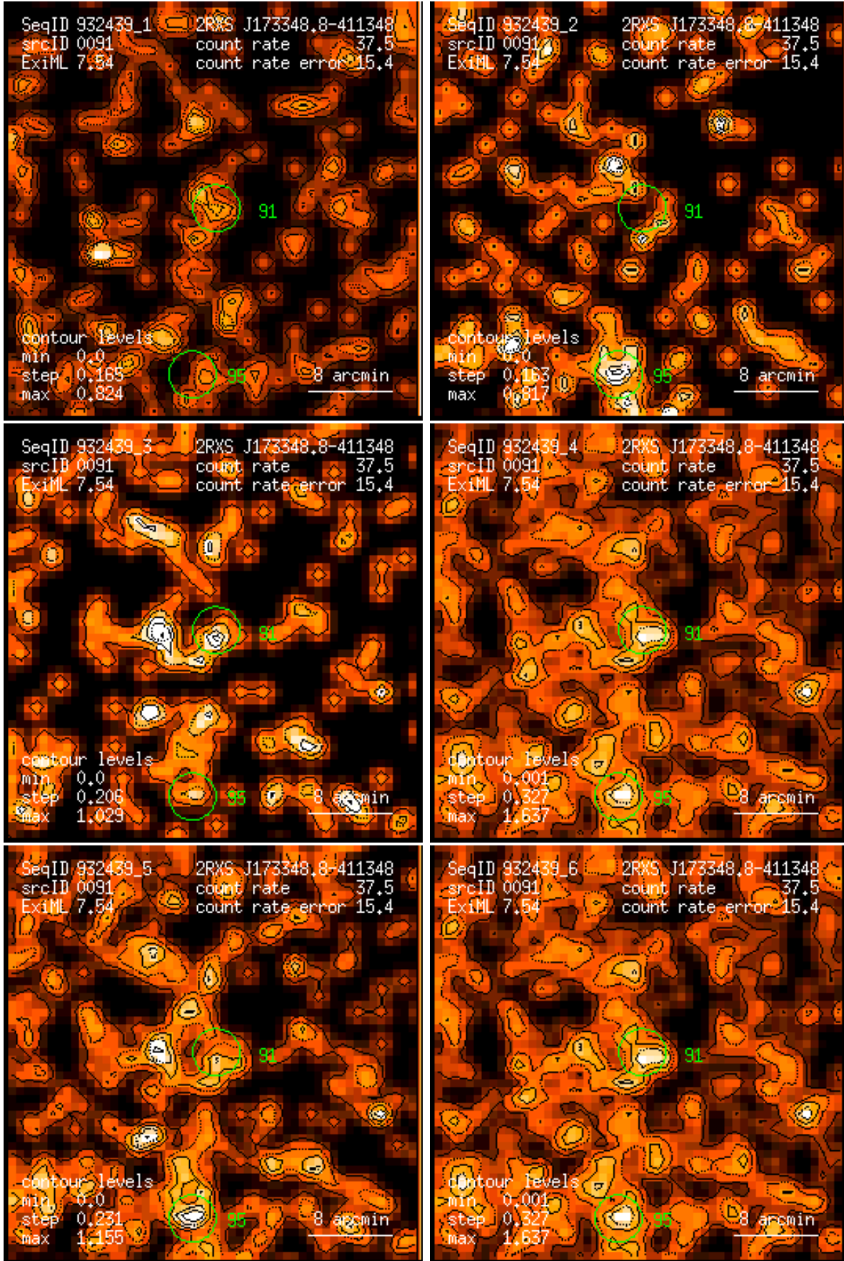
Figure 91: RASS 932439: detection 0091: band rate images, Gaussian filter: (1) PSPC channels 11 – 41, (2) 52 – 90, (3) 91 – 201, (4) 11 – 235, (5) 52 – 201, (6) 11 – 201. Broad band rates in counts/ks. Band rate contour levels in counts/ks/arcmin 2 .
