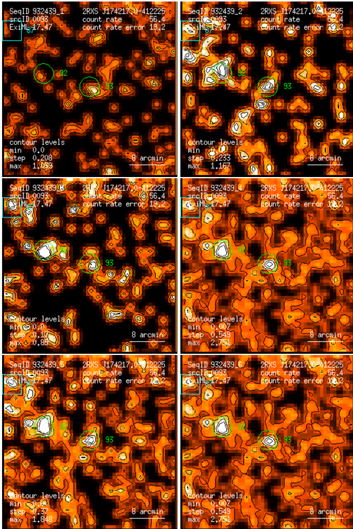
Figure 93: RASS 932439: detection 0093: band rate images, Gaussian filter: (1) PSPC channels 11 – 41, (2) 52 – 90, (3) 91 – 201, (4) 11 – 235, (5) 52 – 201, (6) 11 – 201. Broad band rates in counts/ks. Band rate contour levels in counts/ks/arcmin 2 .
