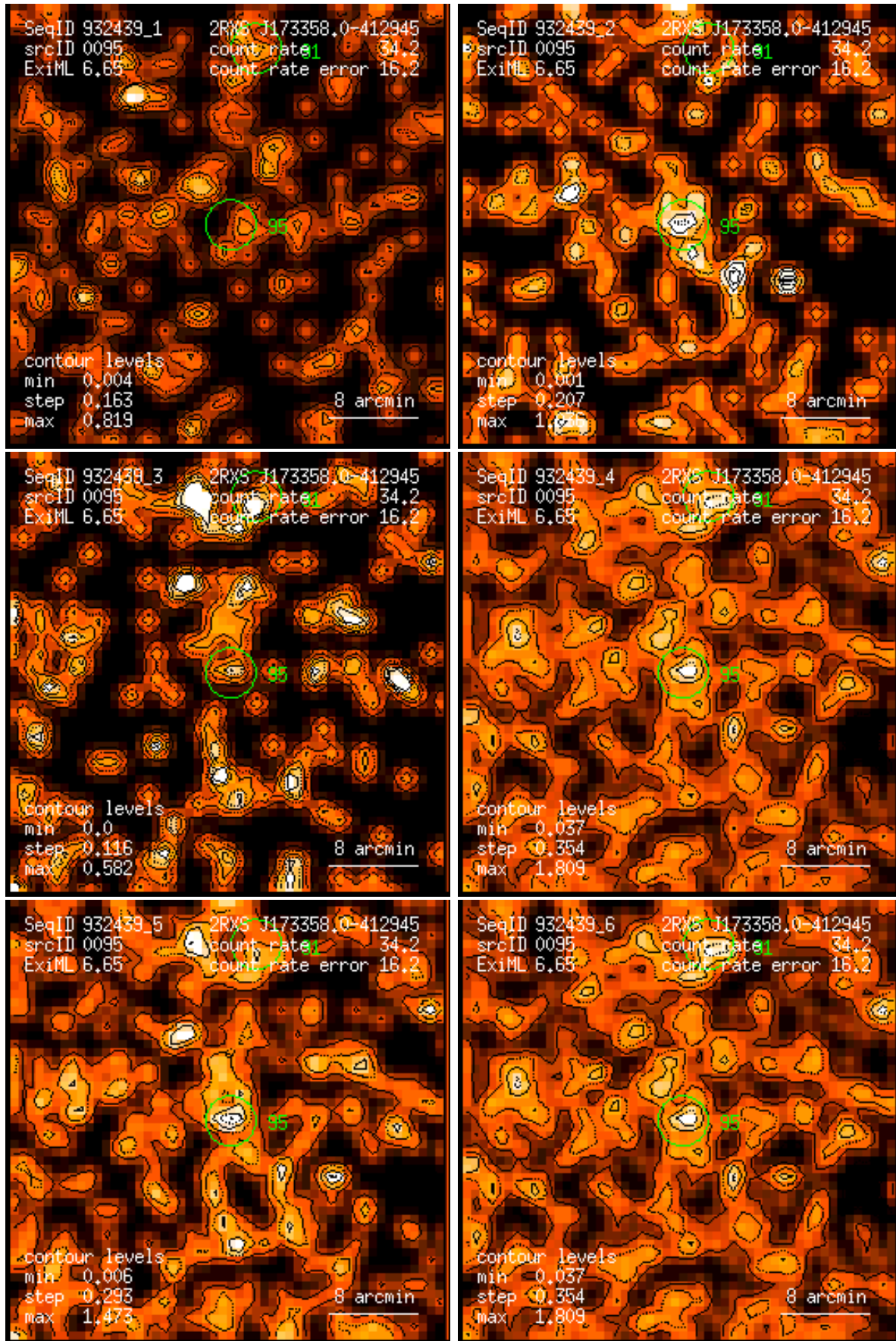
Figure 95: RASS 932439: detection 0095: band rate images, Gaussian filter: (1) PSPC channels 11 – 41, (2) 52 – 90, (3) 91 – 201, (4) 11 – 235, (5) 52 – 201, (6) 11 – 201. Broad band rates in counts/ks. Band rate contour levels in counts/ks/arcmin 2 .
