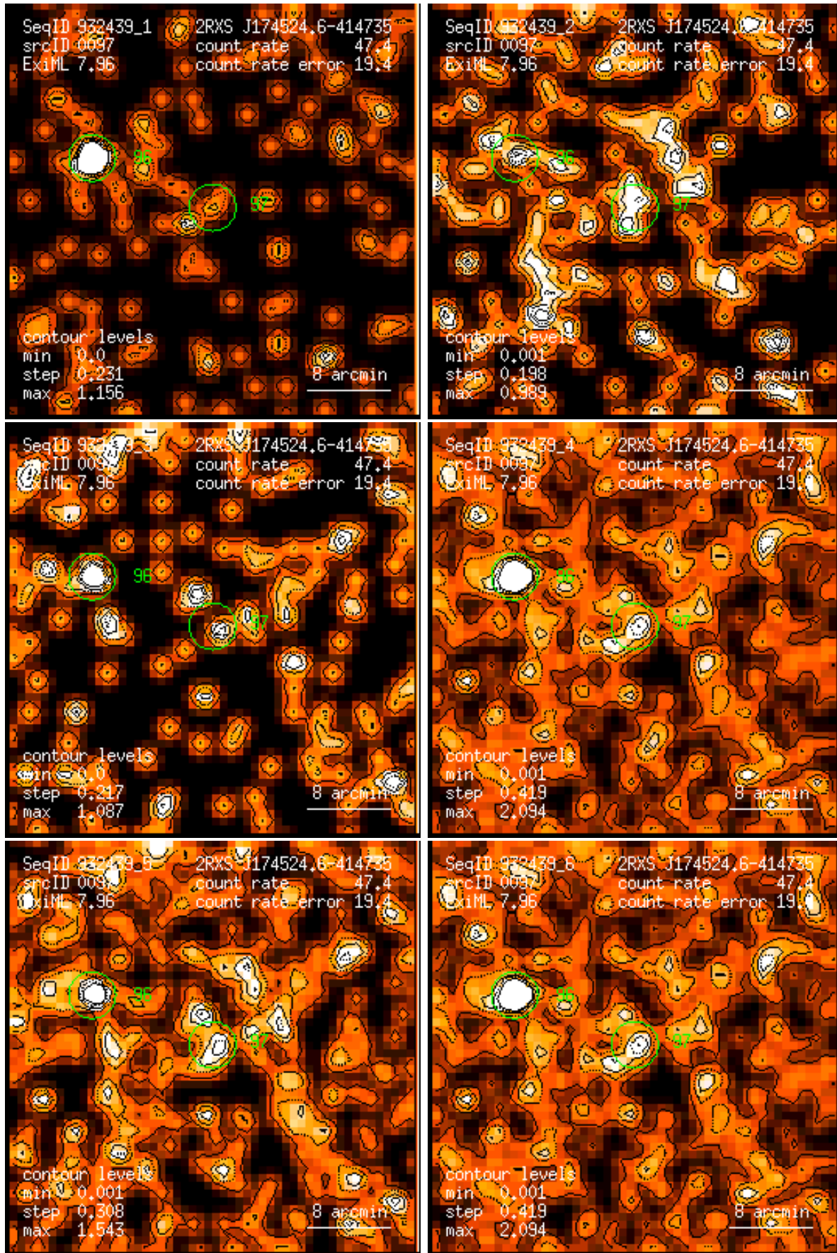
Figure 97: RASS 932439: detection 0097: band rate images, Gaussian filter: (1) PSPC channels 11 – 41, (2) 52 – 90, (3) 91 – 201, (4) 11 – 235, (5) 52 – 201, (6) 11 – 201. Broad band rates in counts/ks. Band rate contour levels in counts/ks/arcmin 2 .
