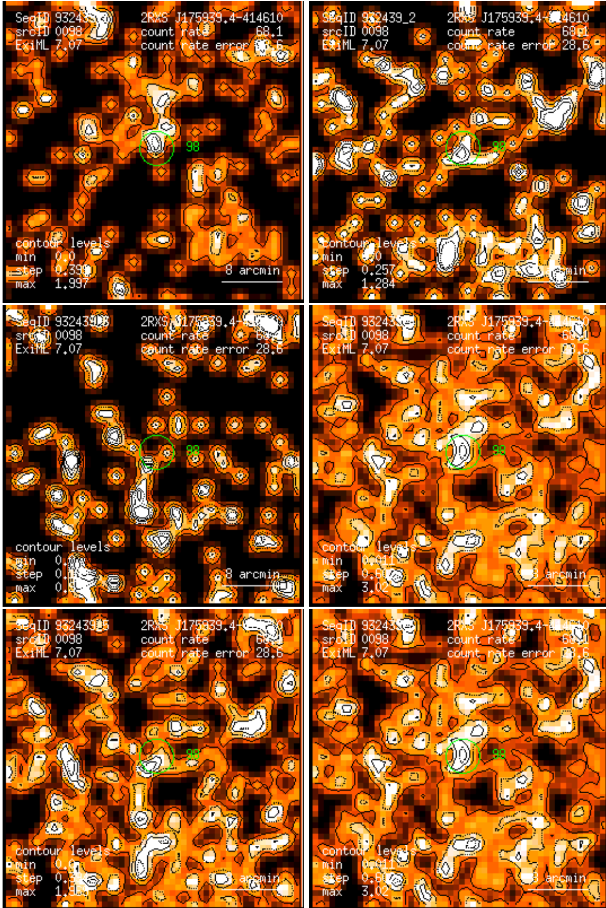
Figure 98: RASS 932439: detection 0098: band rate images, Gaussian filter: (1) PSPC channels 11 – 41, (2) 52 – 90, (3) 91 – 201, (4) 11 – 235, (5) 52 – 201, (6) 11 – 201. Broad band rates in counts/ks. Band rate contour levels in counts/ks/arcmin 2 .
