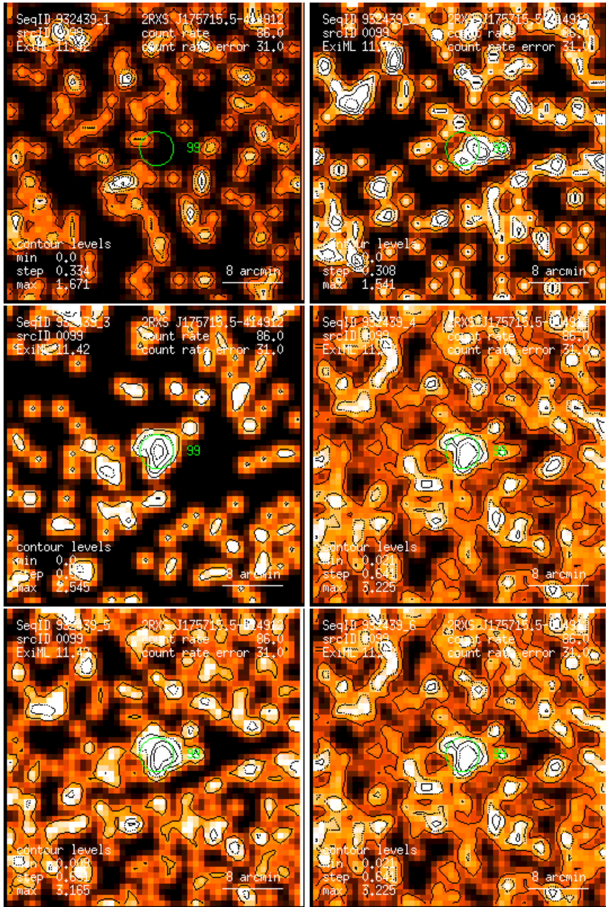
Figure 99: RASS 932439: detection 0099: band rate images, Gaussian filter: (1) PSPC channels 11 – 41, (2) 52 – 90, (3) 91 – 201, (4) 11 – 235, (5) 52 – 201, (6) 11 – 201. Broad band rates in counts/ks. Band rate contour levels in counts/ks/arcmin 2 .
