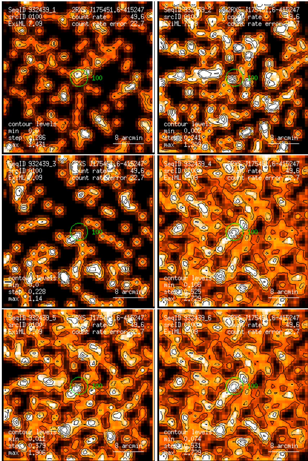
Figure 100: RASS 932439: detection 0100: band rate images, Gaussian filter: (1) PSPC channels 11 – 41, (2) 52 – 90, (3) 91 – 201, (4) 11 – 235, (5) 52 – 201, (6) 11 – 201. Broad band rates in counts/ks. Band rate contour levels in counts/ks/arcmin 2 .
