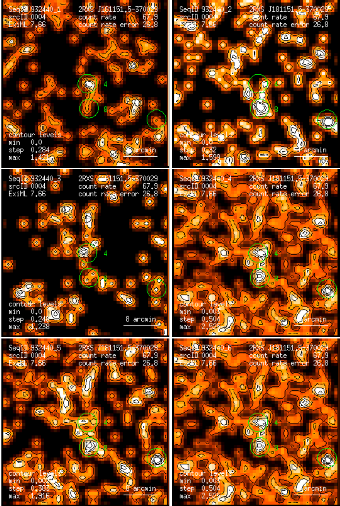
Figure 4: RASS 932440: detection 0004: band rate images, Gaussian filter: (1) PSPC channels 11 – 41, (2) 52 – 90, (3) 91 – 201, (4) 11 – 235, (5) 52 – 201, (6) 11 – 201. Broad band rates in counts/ks. Band rate contour levels in counts/ks/arcmin 2 .
