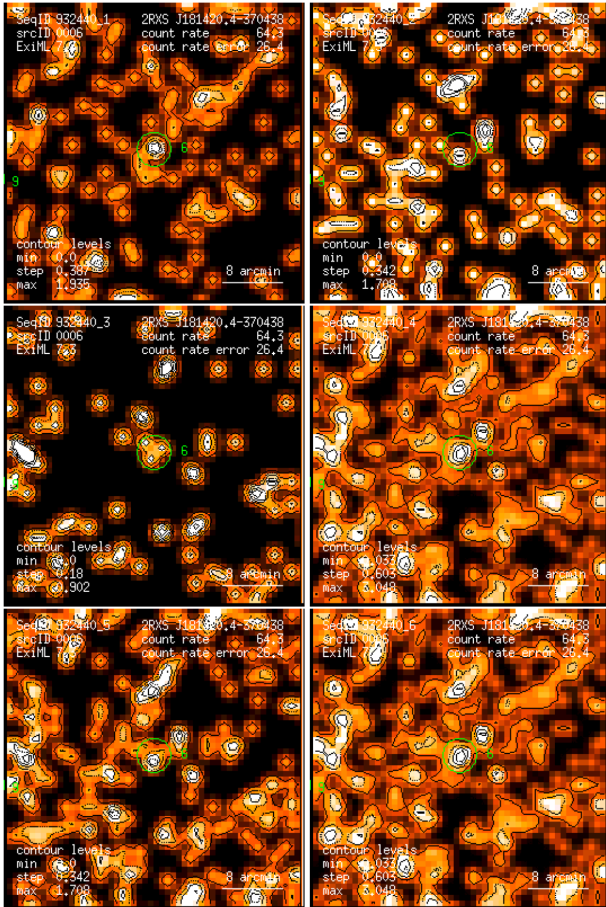
Figure 6: RASS 932440: detection 0006: band rate images, Gaussian filter: (1) PSPC channels 11 – 41, (2) 52 – 90, (3) 91 – 201, (4) 11 – 235, (5) 52 – 201, (6) 11 – 201. Broad band rates in counts/ks. Band rate contour levels in counts/ks/arcmin 2 .
