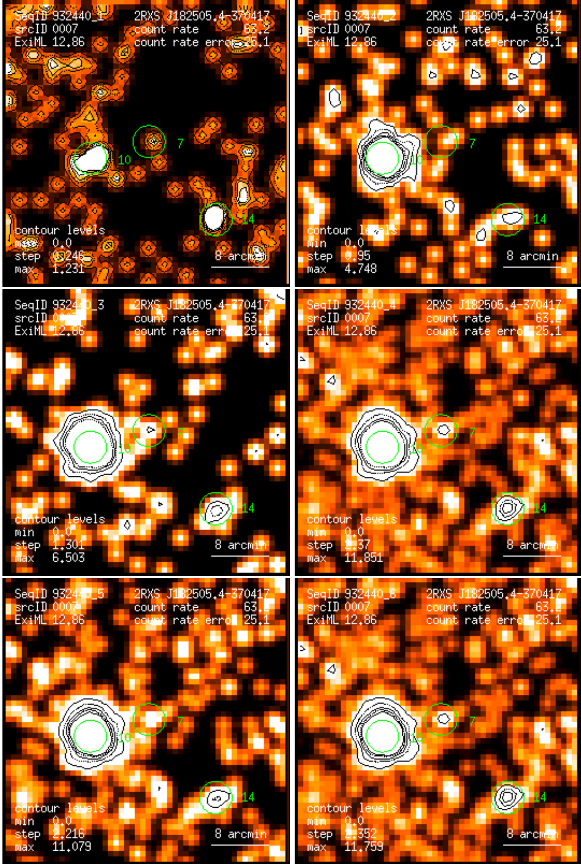
Figure 7: RASS 932440: detection 0007: band rate images, Gaussian filter: (1) PSPC channels 11 – 41, (2) 52 – 90, (3) 91 – 201, (4) 11 – 235, (5) 52 – 201, (6) 11 – 201. Broad band rates in counts/ks. Band rate contour levels in counts/ks/arcmin 2 .
