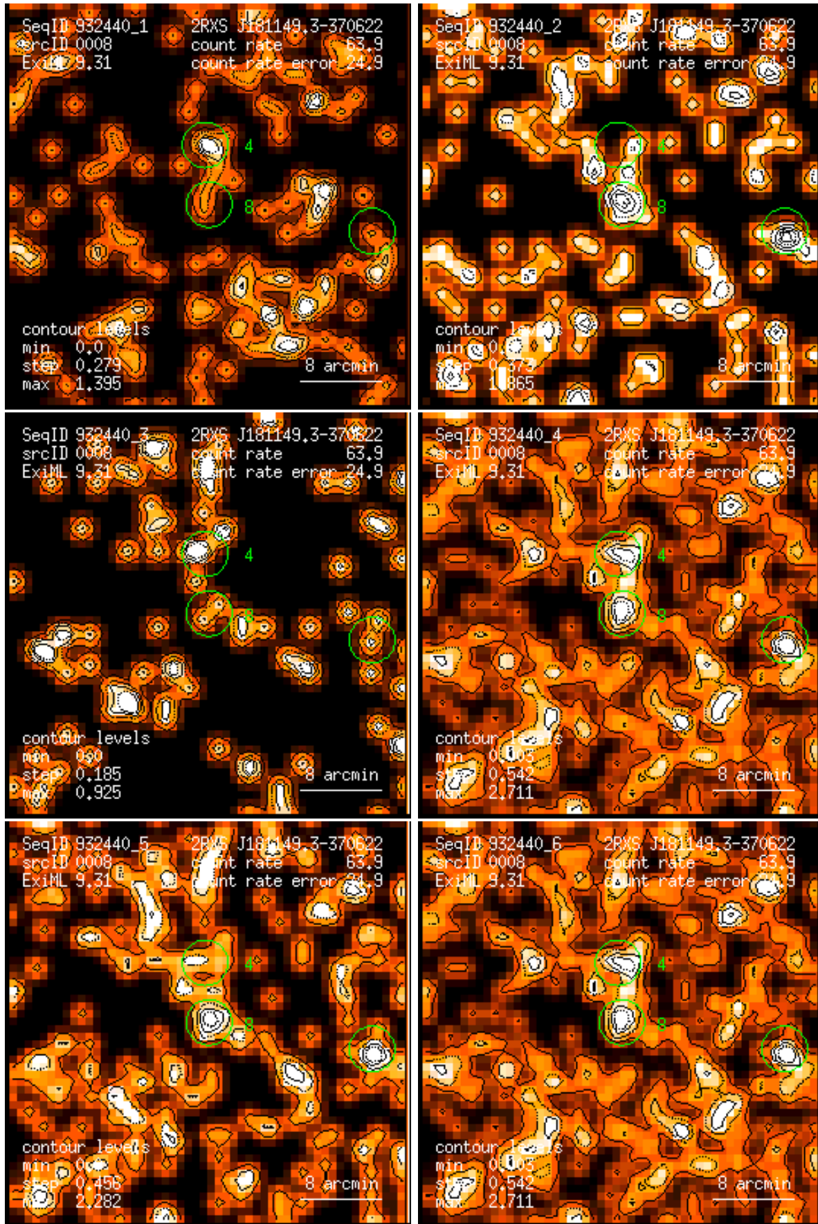
Figure 8: RASS 932440: detection 0008: band rate images, Gaussian filter: (1) PSPC channels 11 – 41, (2) 52 – 90, (3) 91 – 201, (4) 11 – 235, (5) 52 – 201, (6) 11 – 201. Broad band rates in counts/ks. Band rate contour levels in counts/ks/arcmin 2 .
