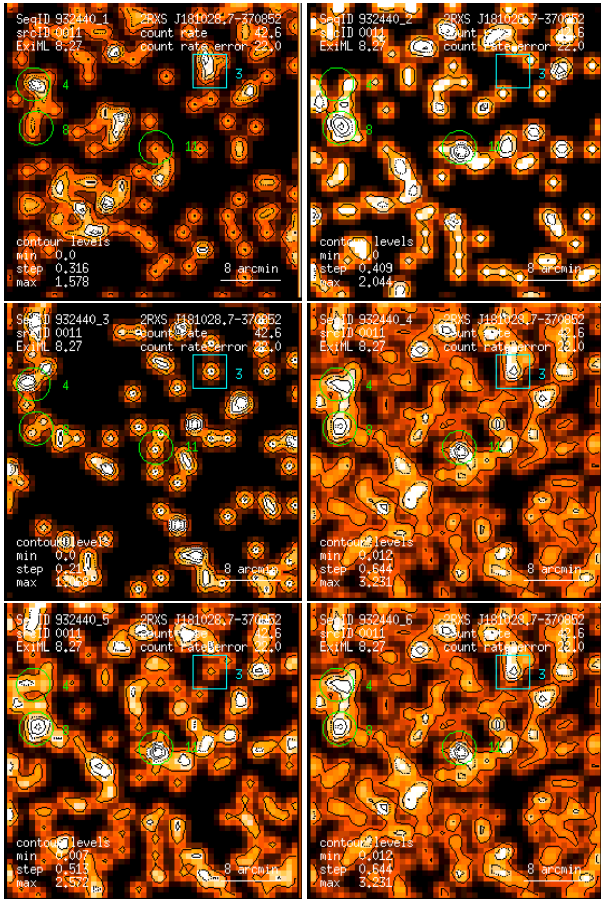
Figure 11: RASS 932440: detection 0011: band rate images, Gaussian filter: (1) PSPC channels 11 – 41, (2) 52 – 90, (3) 91 – 201, (4) 11 – 235, (5) 52 – 201, (6) 11 – 201. Broad band rates in counts/ks. Band rate contour levels in counts/ks/arcmin 2 .
