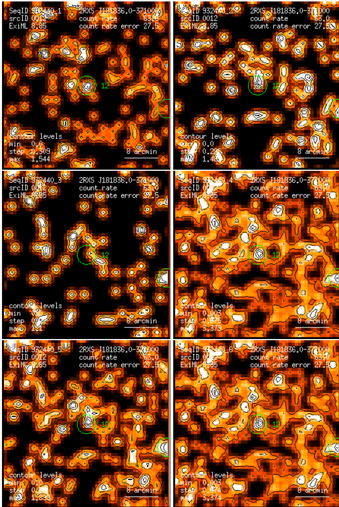
Figure 12: RASS 932440: detection 0012: band rate images, Gaussian filter: (1) PSPC channels 11 – 41, (2) 52 – 90, (3) 91 – 201, (4) 11 – 235, (5) 52 – 201, (6) 11 – 201. Broad band rates in counts/ks. Band rate contour levels in counts/ks/arcmin 2 .
