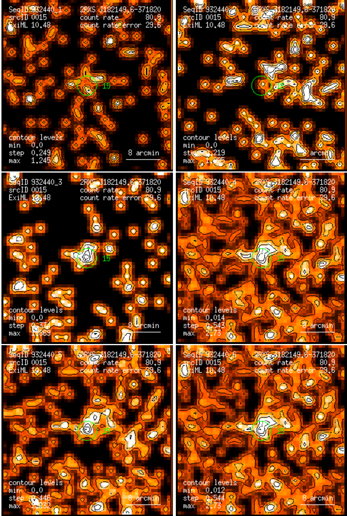
Figure 15: RASS 932440: detection 0015: band rate images, Gaussian filter: (1) PSPC channels 11 – 41, (2) 52 – 90, (3) 91 – 201, (4) 11 – 235, (5) 52 – 201, (6) 11 – 201. Broad band rates in counts/ks. Band rate contour levels in counts/ks/arcmin 2 .
