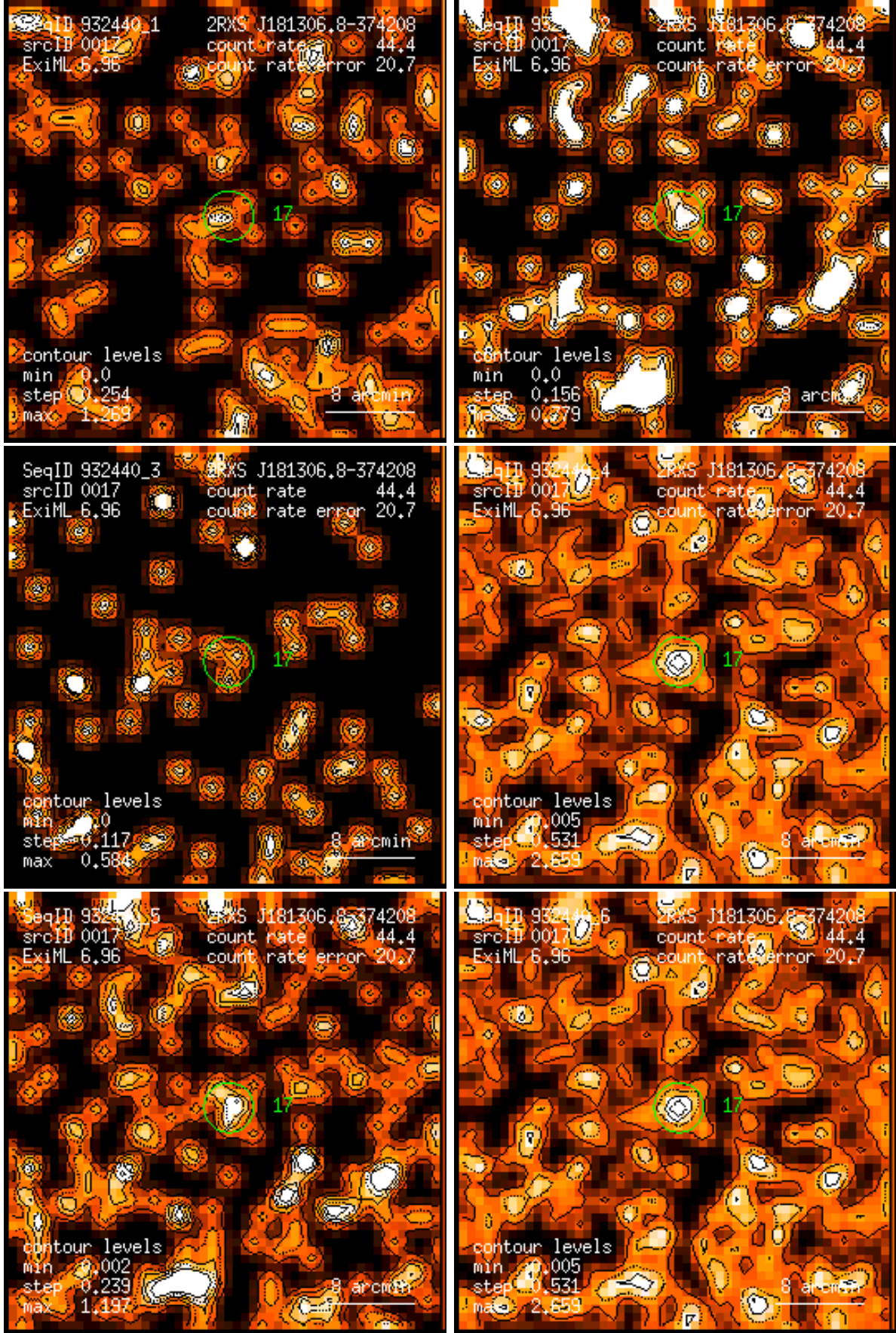
Figure 17: RASS 932440: detection 0017: band rate images, Gaussian filter: (1) PSPC channels 11 – 41, (2) 52 – 90, (3) 91 – 201, (4) 11 – 235, (5) 52 – 201, (6) 11 – 201. Broad band rates in counts/ks. Band rate contour levels in counts/ks/arcmin 2 .
