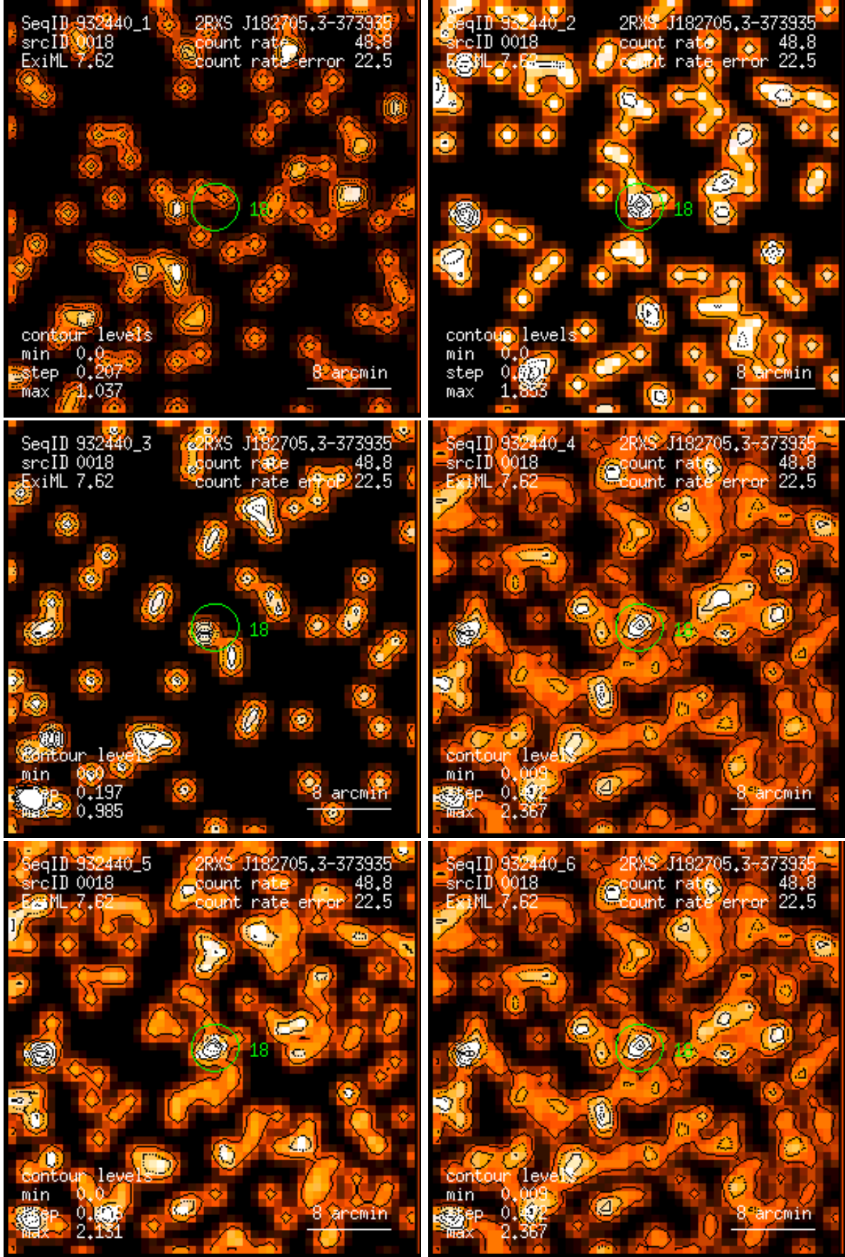
Figure 18: RASS 932440: detection 0018: band rate images, Gaussian filter: (1) PSPC channels 11 – 41, (2) 52 – 90, (3) 91 – 201, (4) 11 – 235, (5) 52 – 201, (6) 11 – 201. Broad band rates in counts/ks. Band rate contour levels in counts/ks/arcmin 2 .
