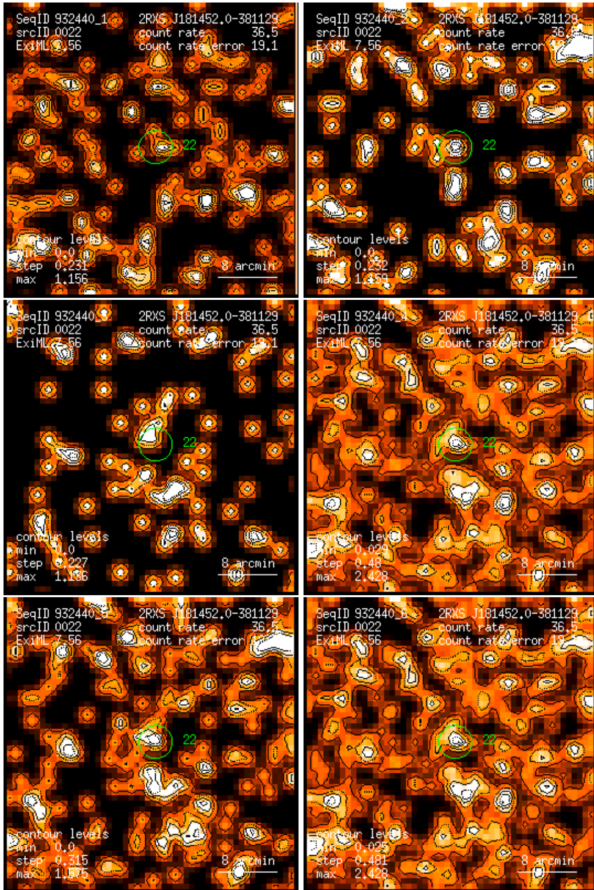
Figure 22: RASS 932440: detection 0022: band rate images, Gaussian filter: (1) PSPC channels 11 – 41, (2) 52 – 90, (3) 91 – 201, (4) 11 – 235, (5) 52 – 201, (6) 11 – 201. Broad band rates in counts/ks. Band rate contour levels in counts/ks/arcmin 2 .
