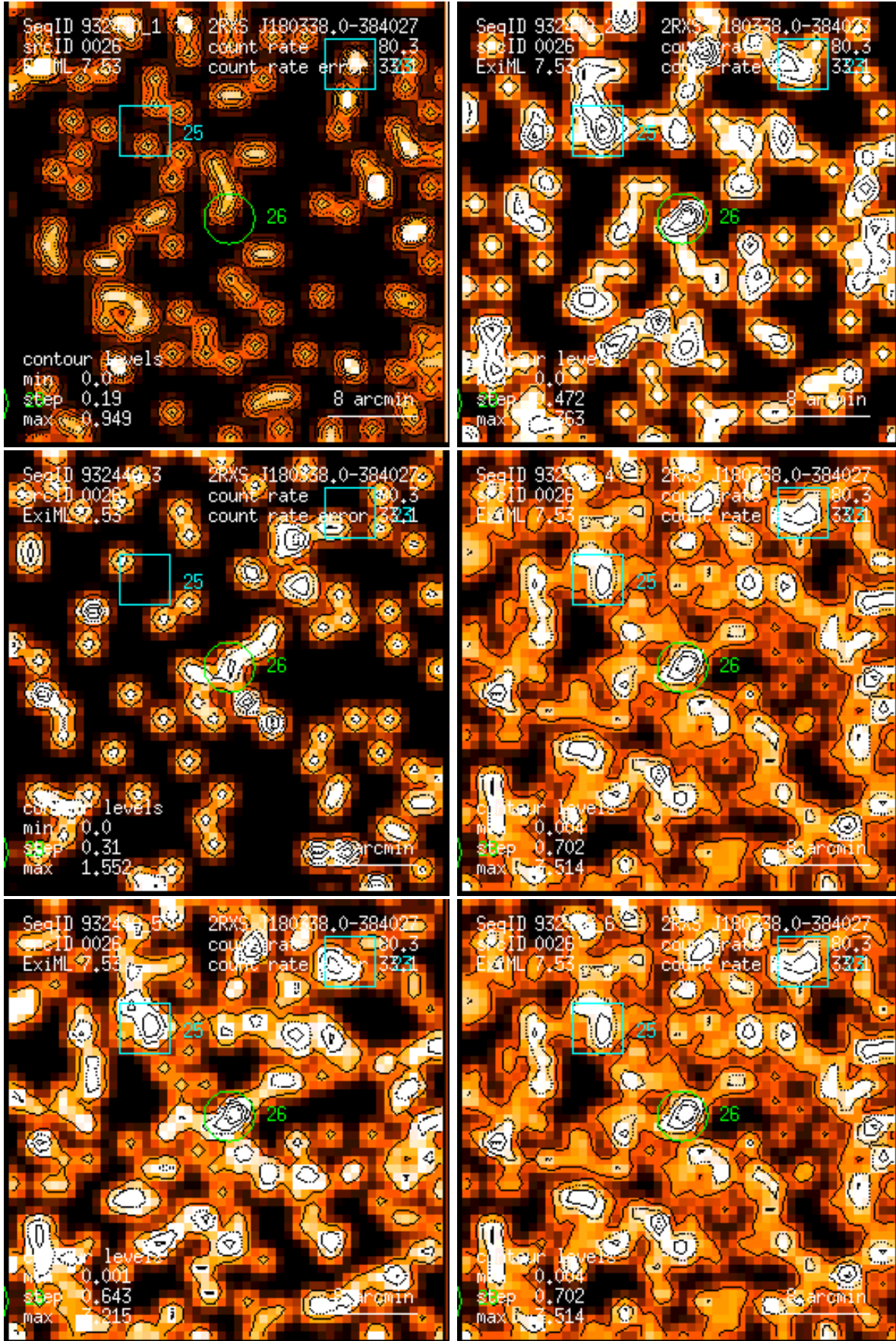
Figure 26: RASS 932440: detection 0026: band rate images, Gaussian filter: (1) PSPC channels 11 – 41, (2) 52 – 90, (3) 91 – 201, (4) 11 – 235, (5) 52 – 201, (6) 11 – 201. Broad band rates in counts/ks. Band rate contour levels in counts/ks/arcmin 2 .
