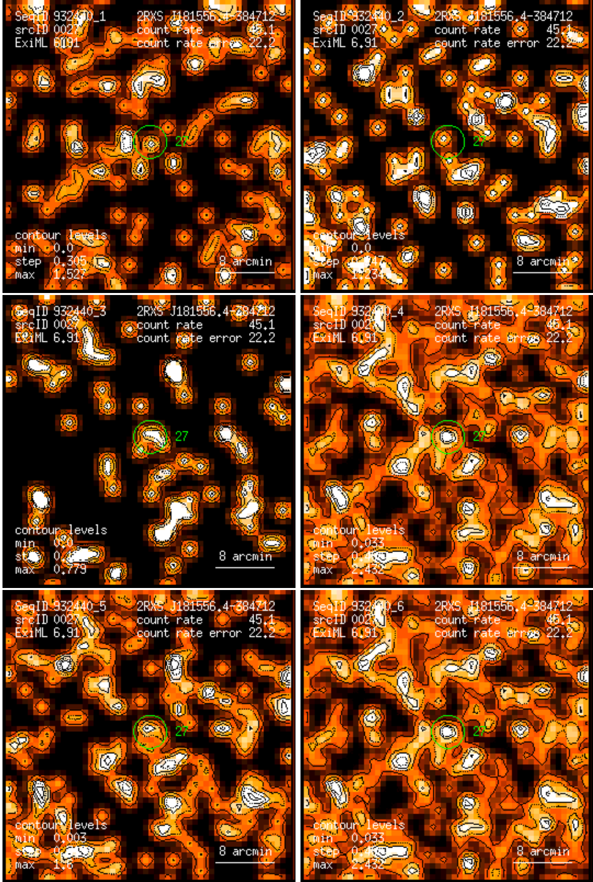
Figure 27: RASS 932440: detection 0027: band rate images, Gaussian filter: (1) PSPC channels 11 – 41, (2) 52 – 90, (3) 91 – 201, (4) 11 – 235, (5) 52 – 201, (6) 11 – 201. Broad band rates in counts/ks. Band rate contour levels in counts/ks/arcmin 2 .
