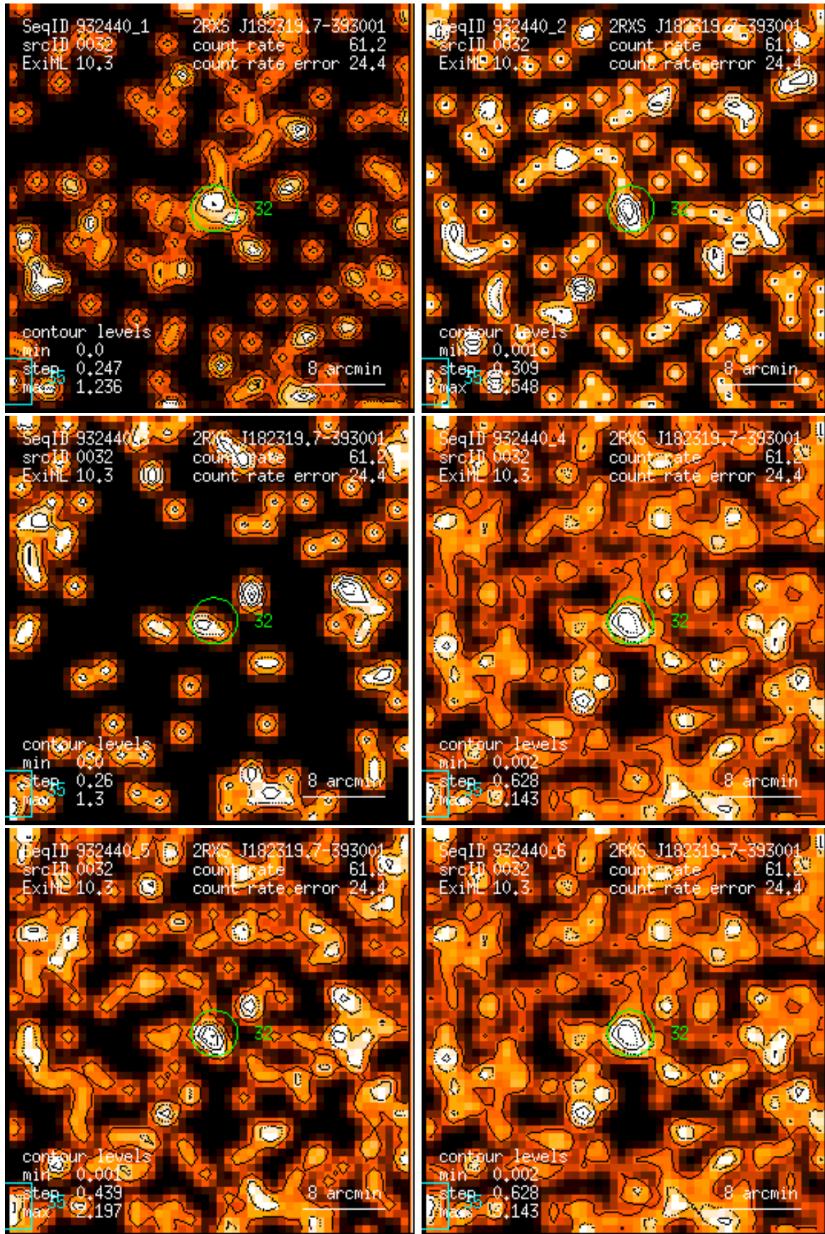
Figure 32: RASS 932440: detection 0032: band rate images, Gaussian filter: (1) PSPC channels 11 – 41, (2) 52 – 90, (3) 91 – 201, (4) 11 – 235, (5) 52 – 201, (6) 11 – 201. Broad band rates in counts/ks. Band rate contour levels in counts/ks/arcmin 2 .
