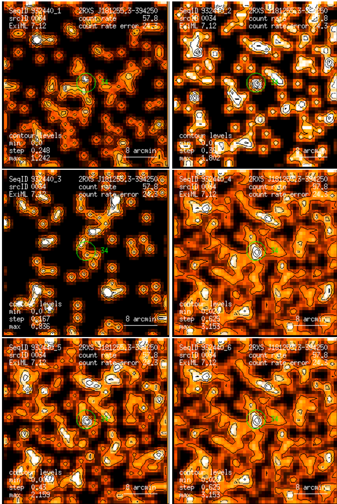
Figure 34: RASS 932440: detection 0034: band rate images, Gaussian filter: (1) PSPC channels 11 – 41, (2) 52 – 90, (3) 91 – 201, (4) 11 – 235, (5) 52 – 201, (6) 11 – 201. Broad band rates in counts/ks. Band rate contour levels in counts/ks/arcmin 2 .
