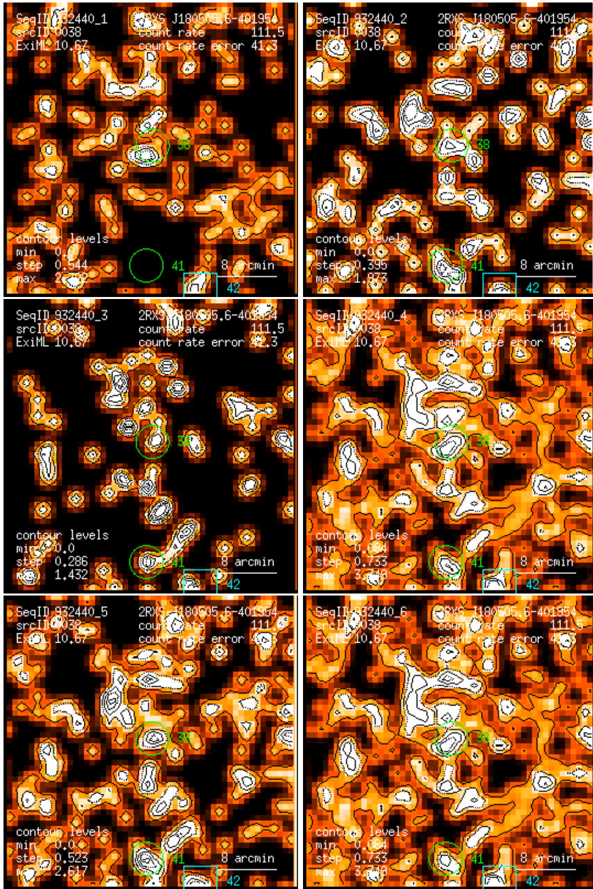
Figure 38: RASS 932440: detection 0038: band rate images, Gaussian filter: (1) PSPC channels 11 – 41, (2) 52 – 90, (3) 91 – 201, (4) 11 – 235, (5) 52 – 201, (6) 11 – 201. Broad band rates in counts/ks. Band rate contour levels in counts/ks/arcmin 2 .
