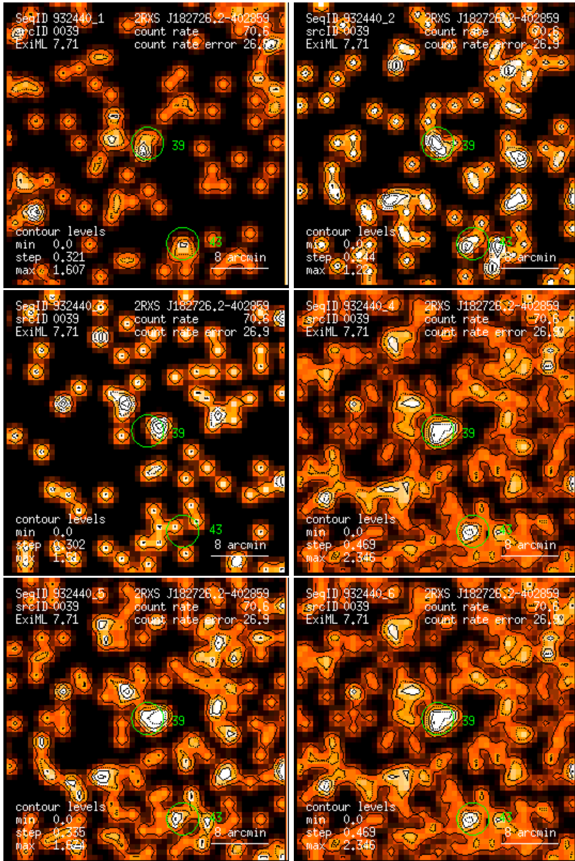
Figure 39: RASS 932440: detection 0039: band rate images, Gaussian filter: (1) PSPC channels 11 – 41, (2) 52 – 90, (3) 91 – 201, (4) 11 – 235, (5) 52 – 201, (6) 11 – 201. Broad band rates in counts/ks. Band rate contour levels in counts/ks/arcmin 2 .
