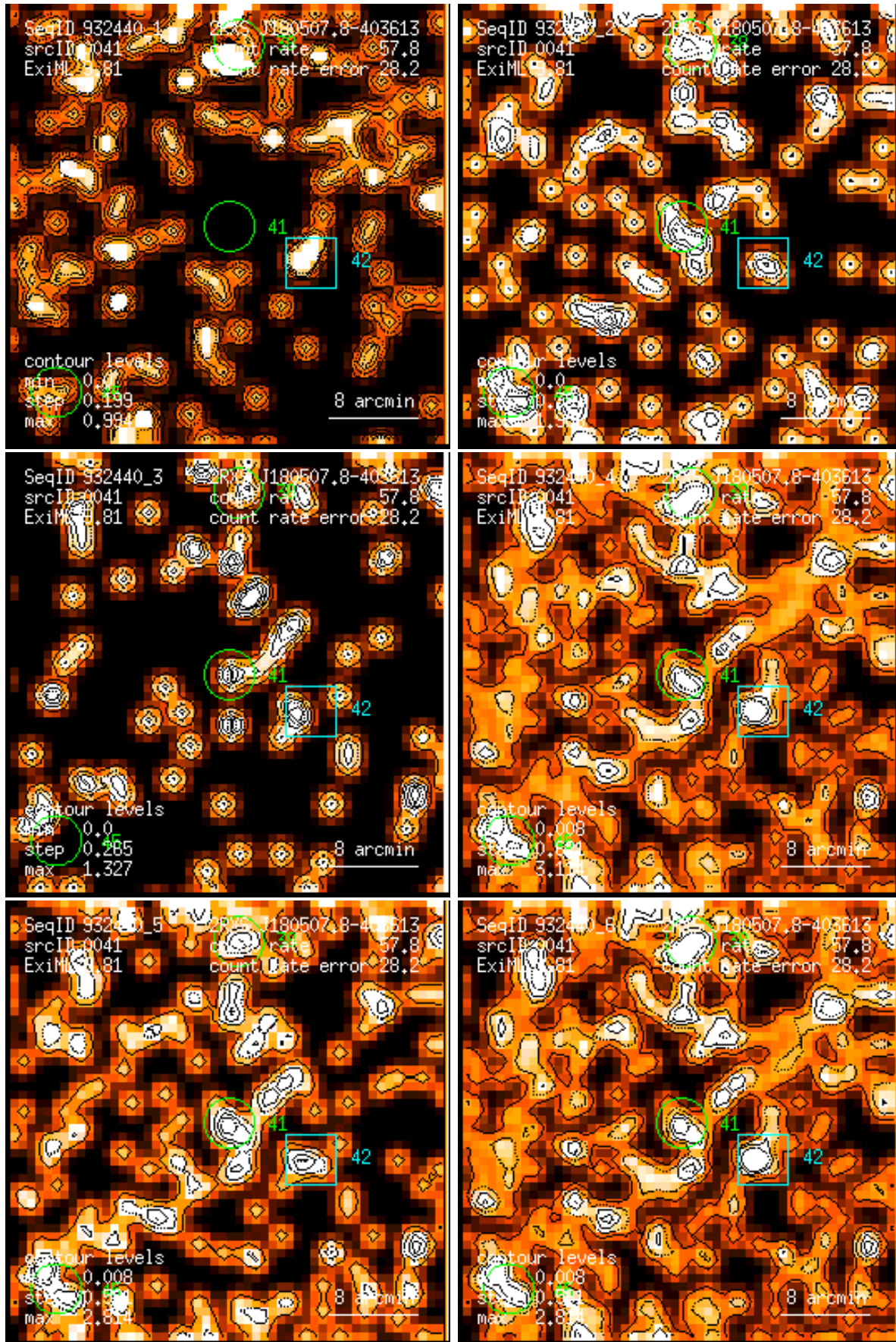
Figure 41: RASS 932440: detection 0041: band rate images, Gaussian filter: (1) PSPC channels 11 – 41, (2) 52 – 90, (3) 91 – 201, (4) 11 – 235, (5) 52 – 201, (6) 11 – 201. Broad band rates in counts/ks. Band rate contour levels in counts/ks/arcmin 2 .
